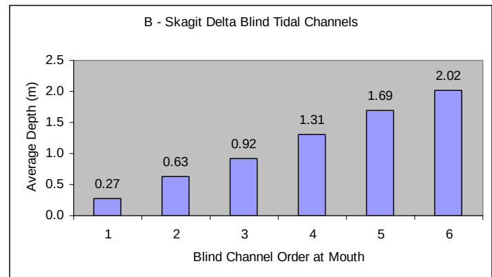
Figure D.III.3. (A) Frequency distribution of Skagit delta blind channels by order at their mouth. (B) Average depth of Skagit delta blind channels by order at their mouth.
