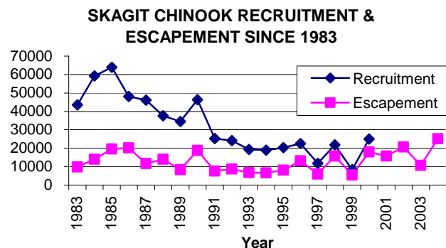
Figure 1.2. Trends in total (spring, summer, and fall) Chinook recruitment and escapement since 1983. Recruitment numbers are from post-season runs using FRAM.
