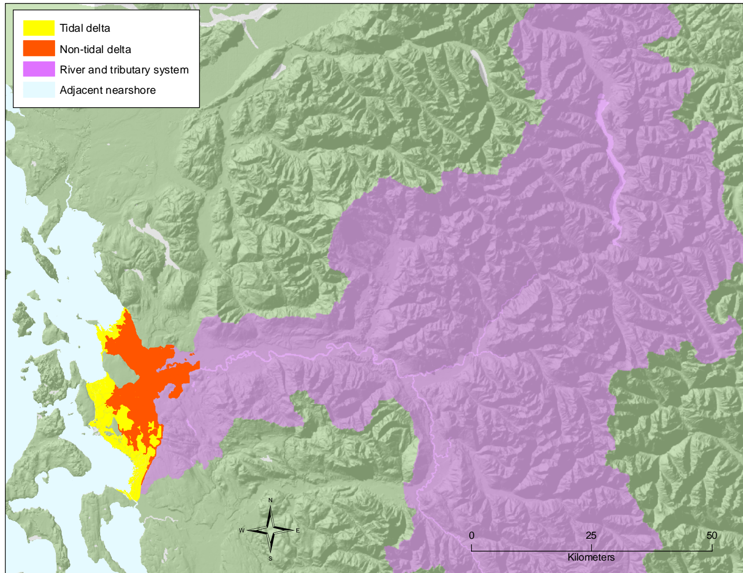
Figure 8.1. Geomorphic regions of the Skagit Basin.
