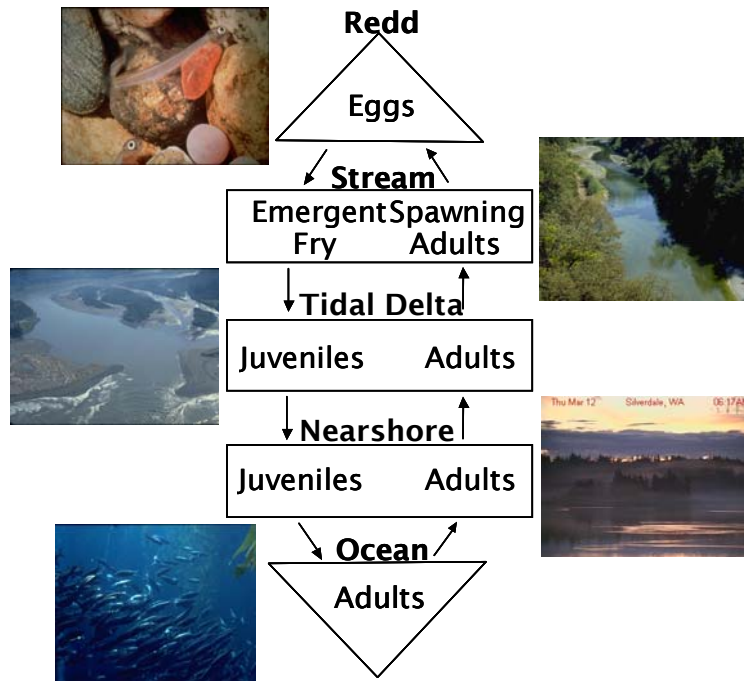
Figure 5.1. Chinook life cycle model . Each life stage produces recruits for the next stage.
