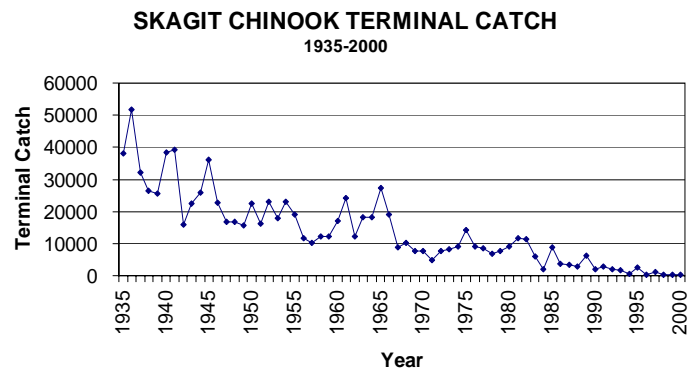
Figure 1.1. Chinook net catch since 1935 in Skagit Bay and River.
