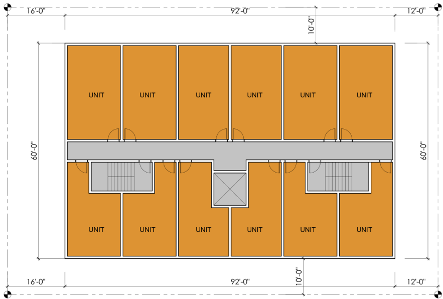
LEVEL 3-5
