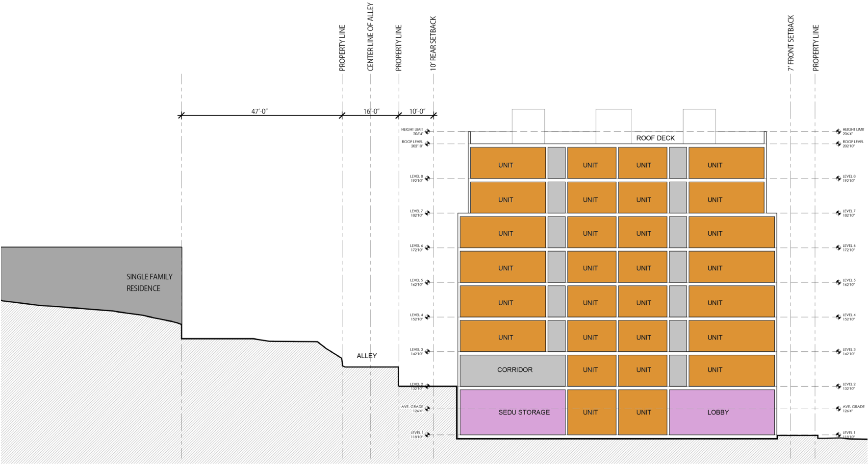
CROSS SECTION
