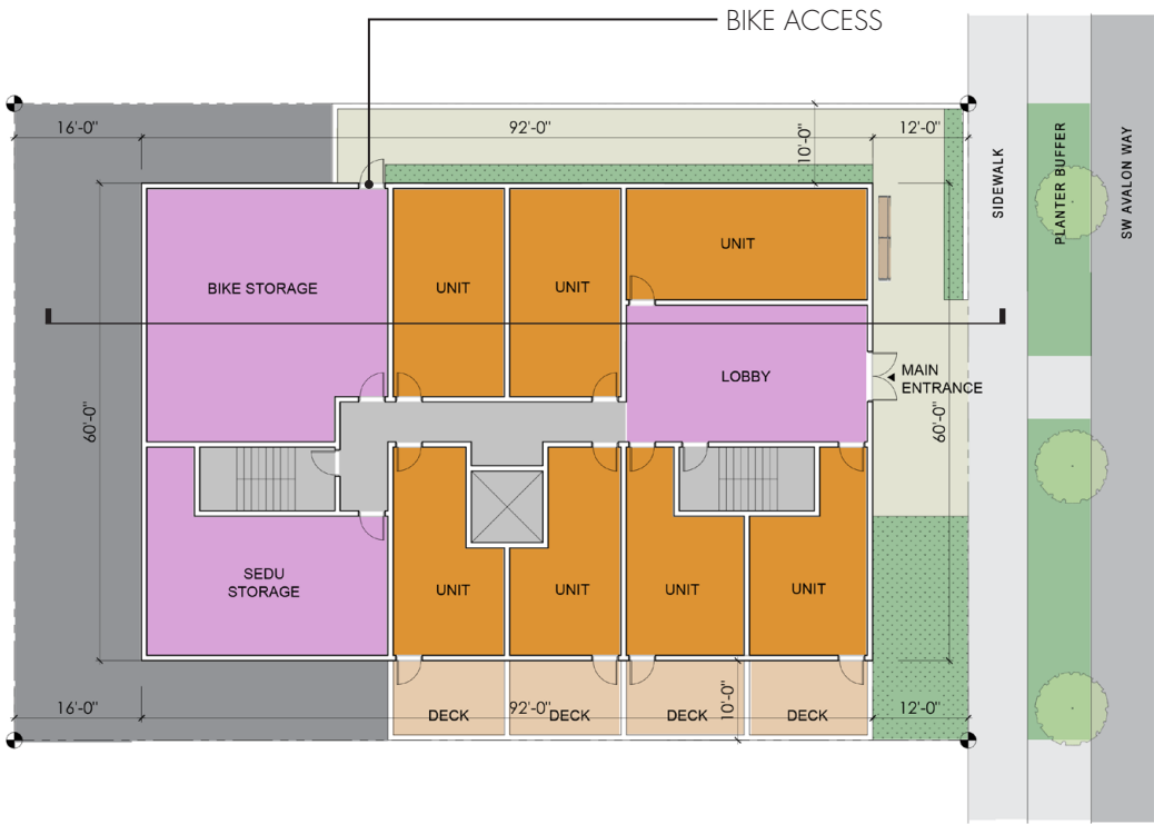
GROUND LEVEL
