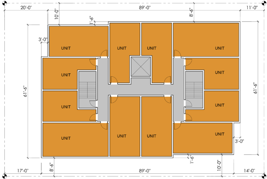
LEVEL 3-6
