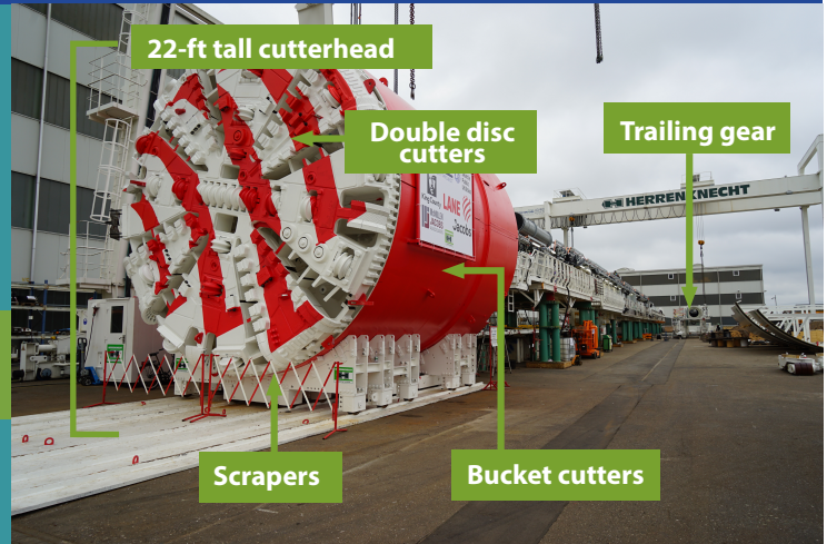
These are key pieces of the TBM that will be used to build the Ship Canal storage tunnel.
