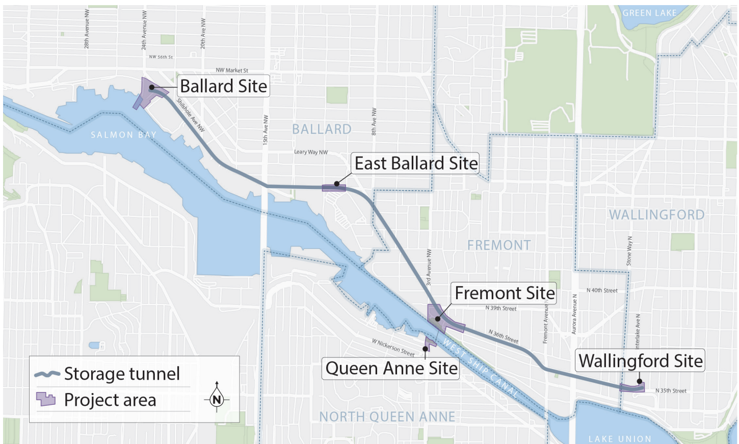
The Ship Canal water quality tunnel will span from Ballard to Wallingford.
