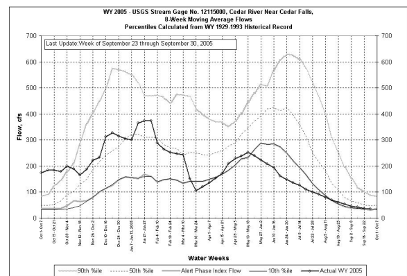
Figure 3. Real-time HCP Alert Phase reservoir index inflow switching criteria monitoring and tracking graph for the reporting period October 1, 2004 to September 30, 2005 (i.e., Water Year 2005).
