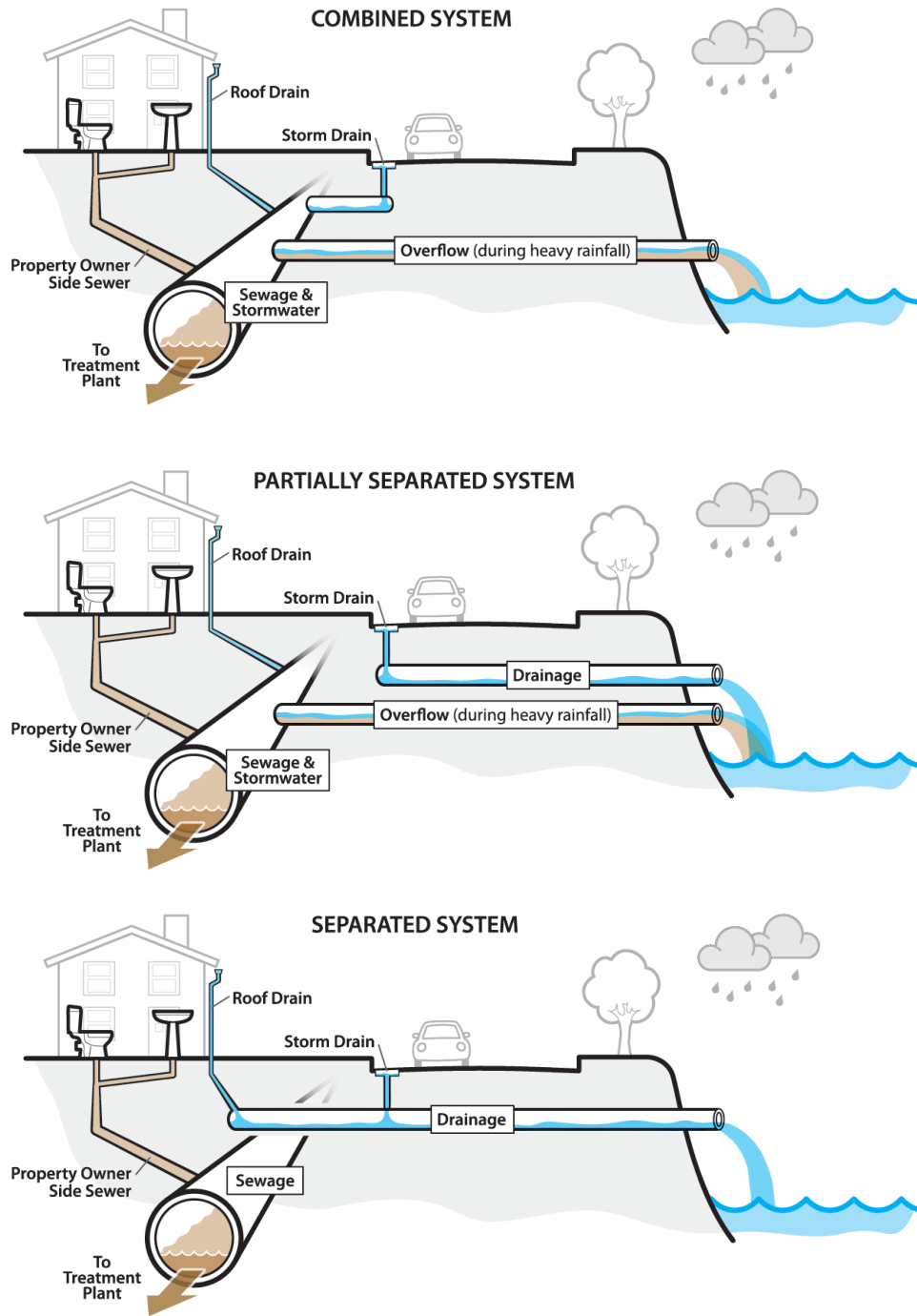
Figure I.1-2 Combined, Separated and Partially Separated Systems
