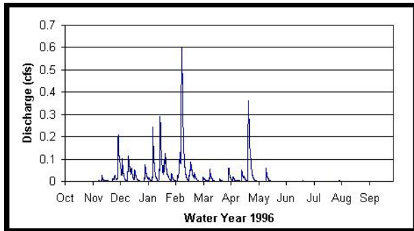
Figure F.4. Runoff from 10-acre Forested Site.
