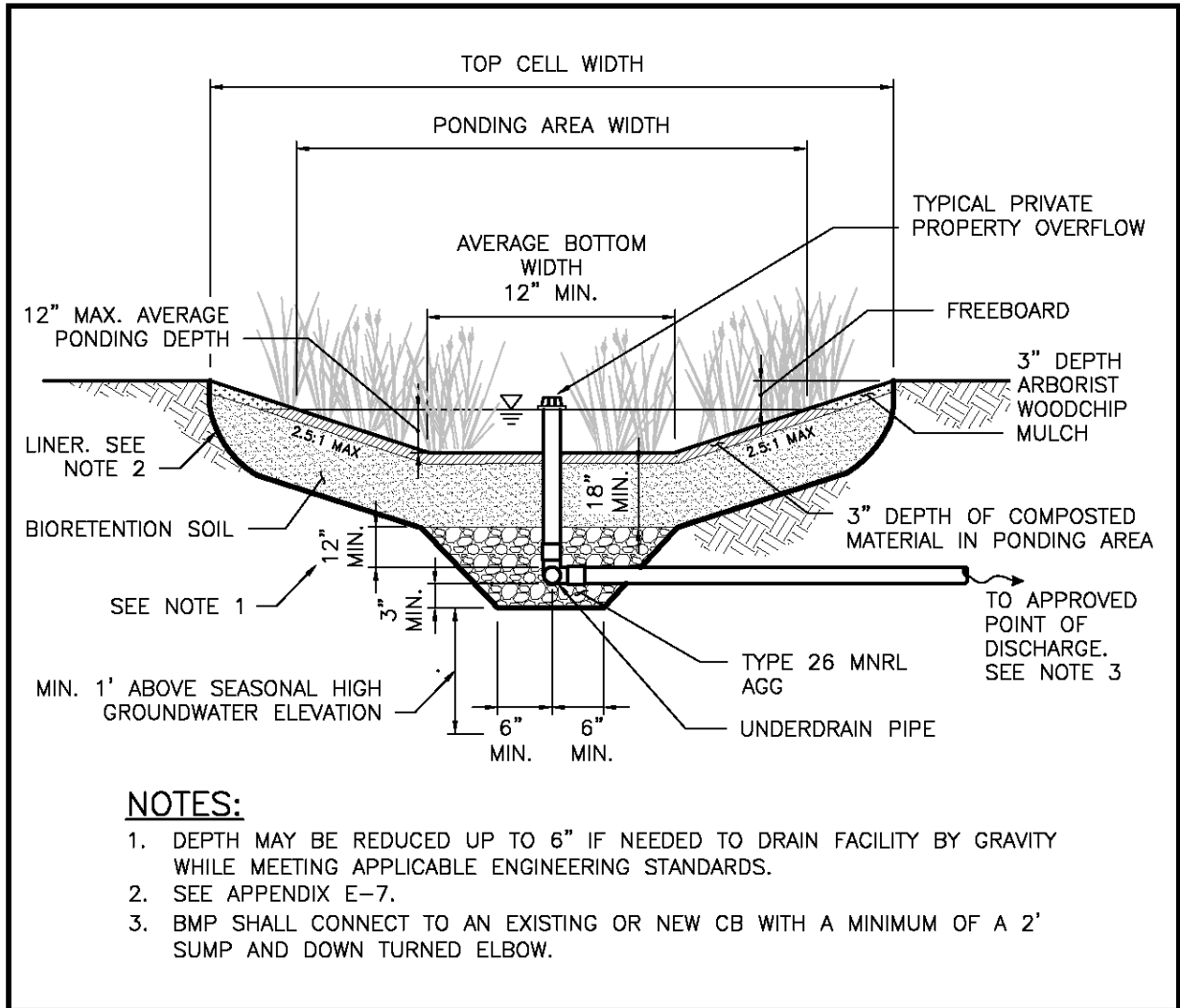
Figure 5.29. Non-infiltrating Bioretention Facility with Sloped Sides.
