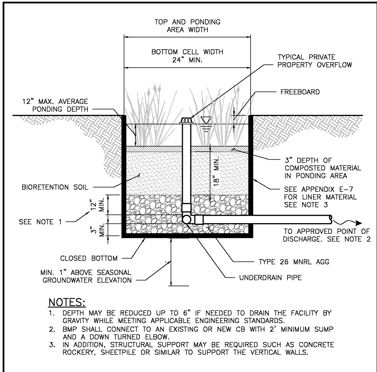
Figure 5.30. Non-infiltrating Bioretention Facility with Vertical Sides.
