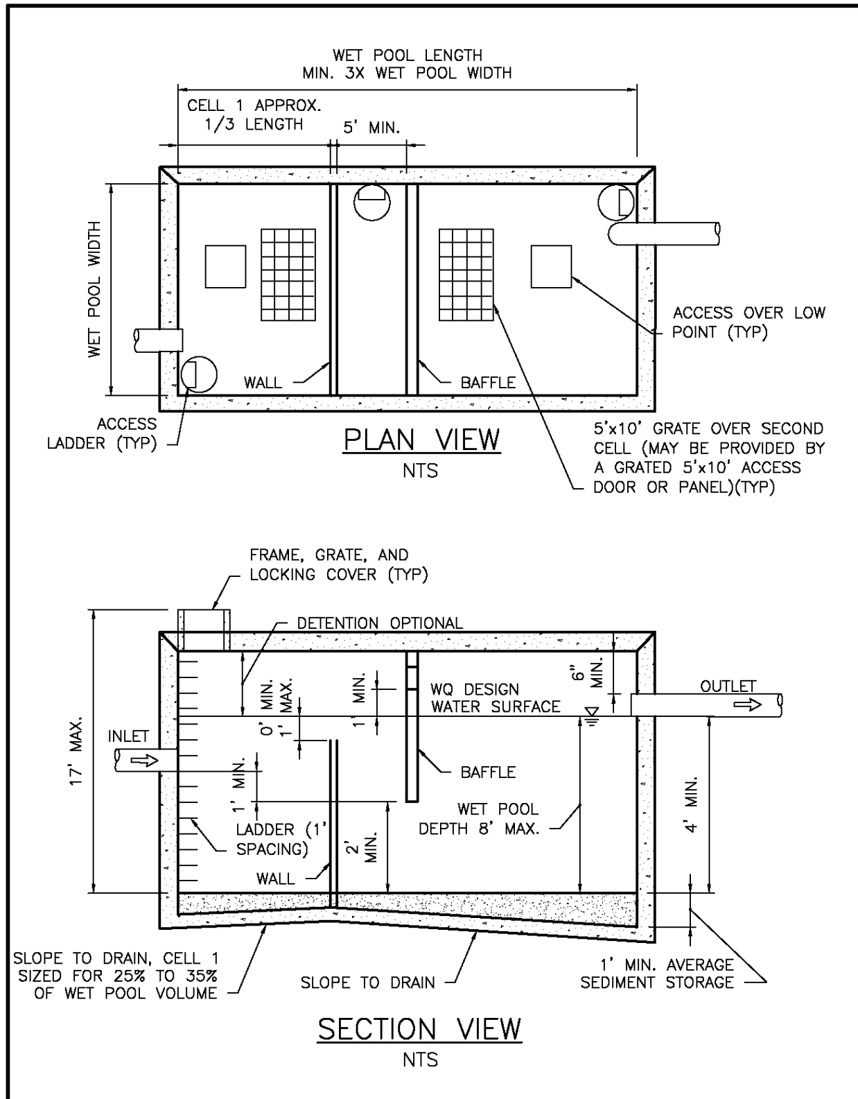
Figure 5.32. Typical Wet Vault.
