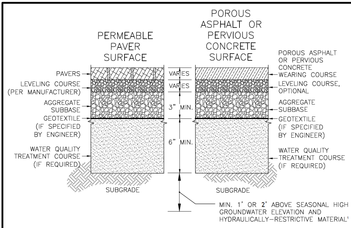
Figure 5.25. Permeable Pavement Surface.
