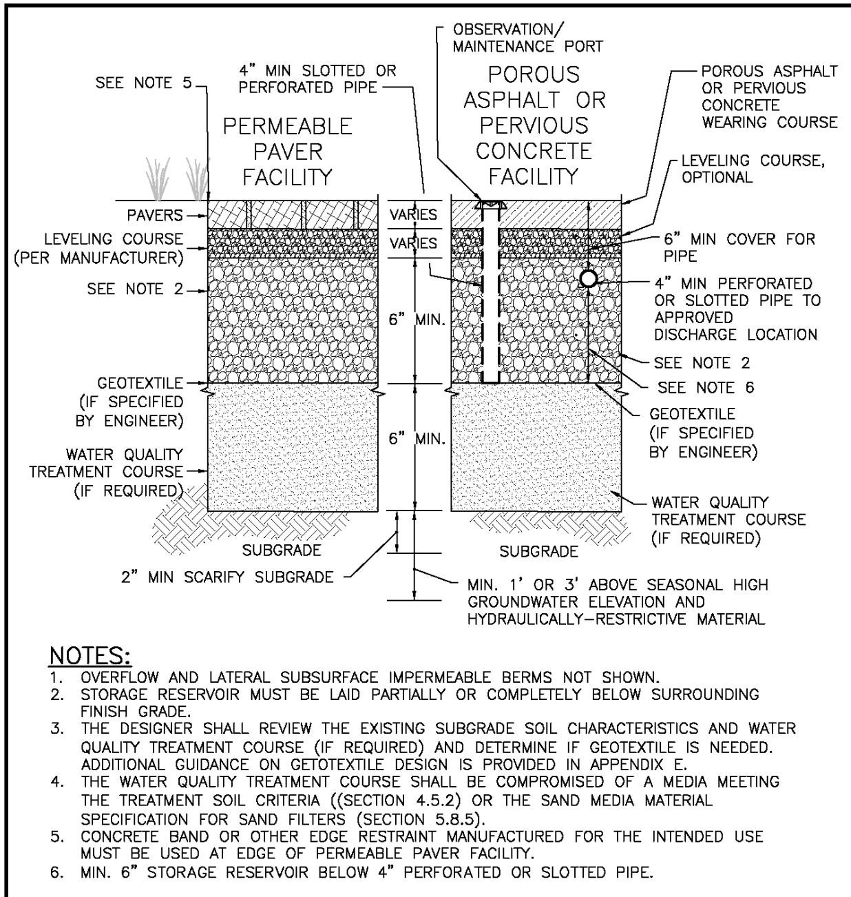
Figure 5.17. Permeable Pavement Facility.
