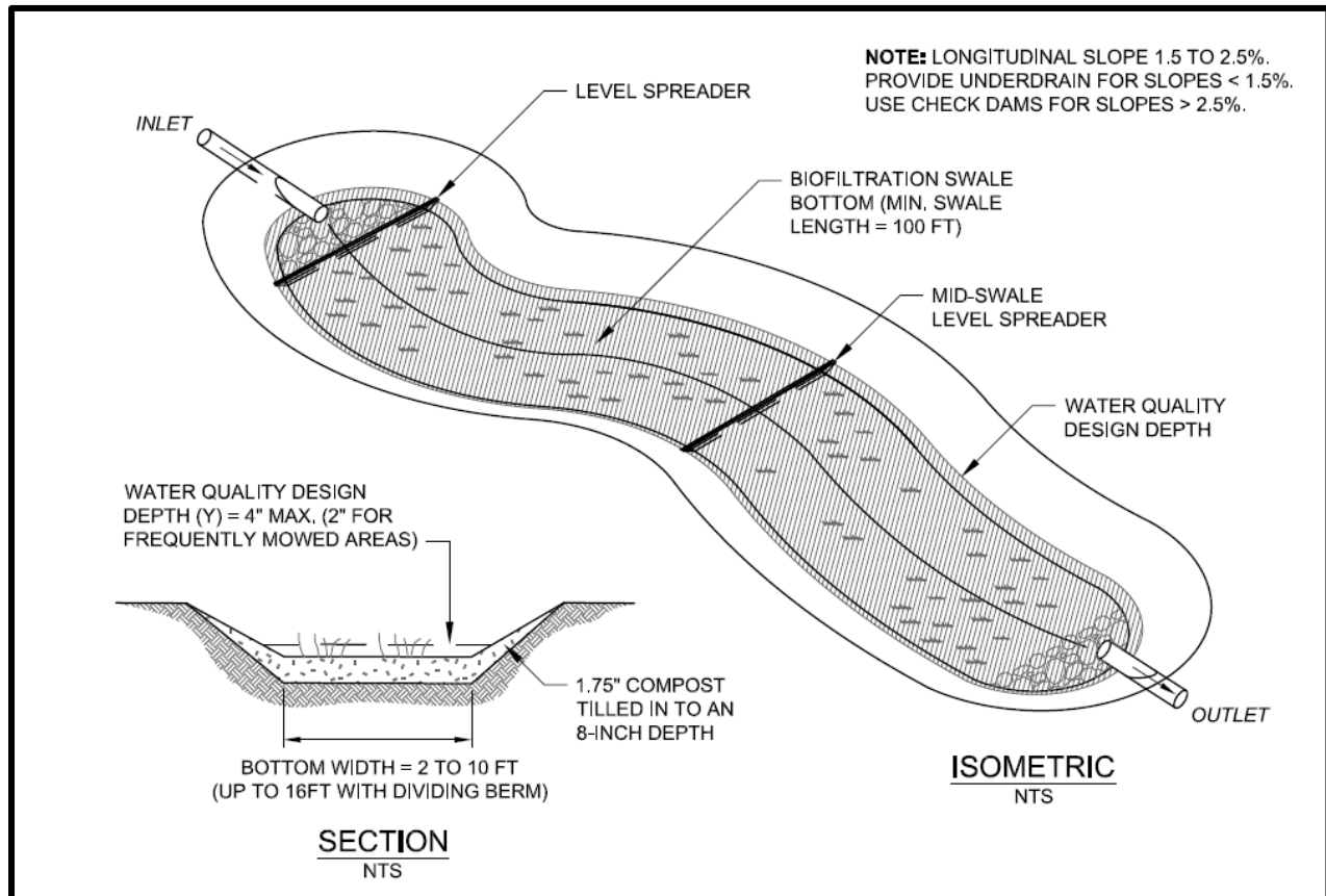
Figure 5.31. Biofiltration Swale Plan and Profile.
