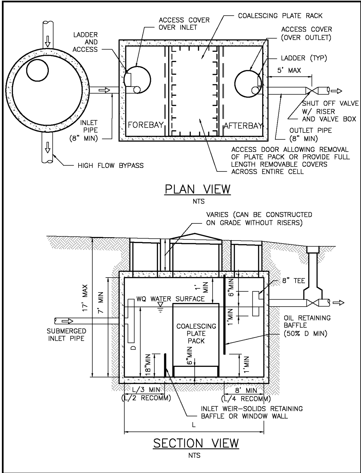
Figure 5.34. Typical Coalescing Plate Separator.
