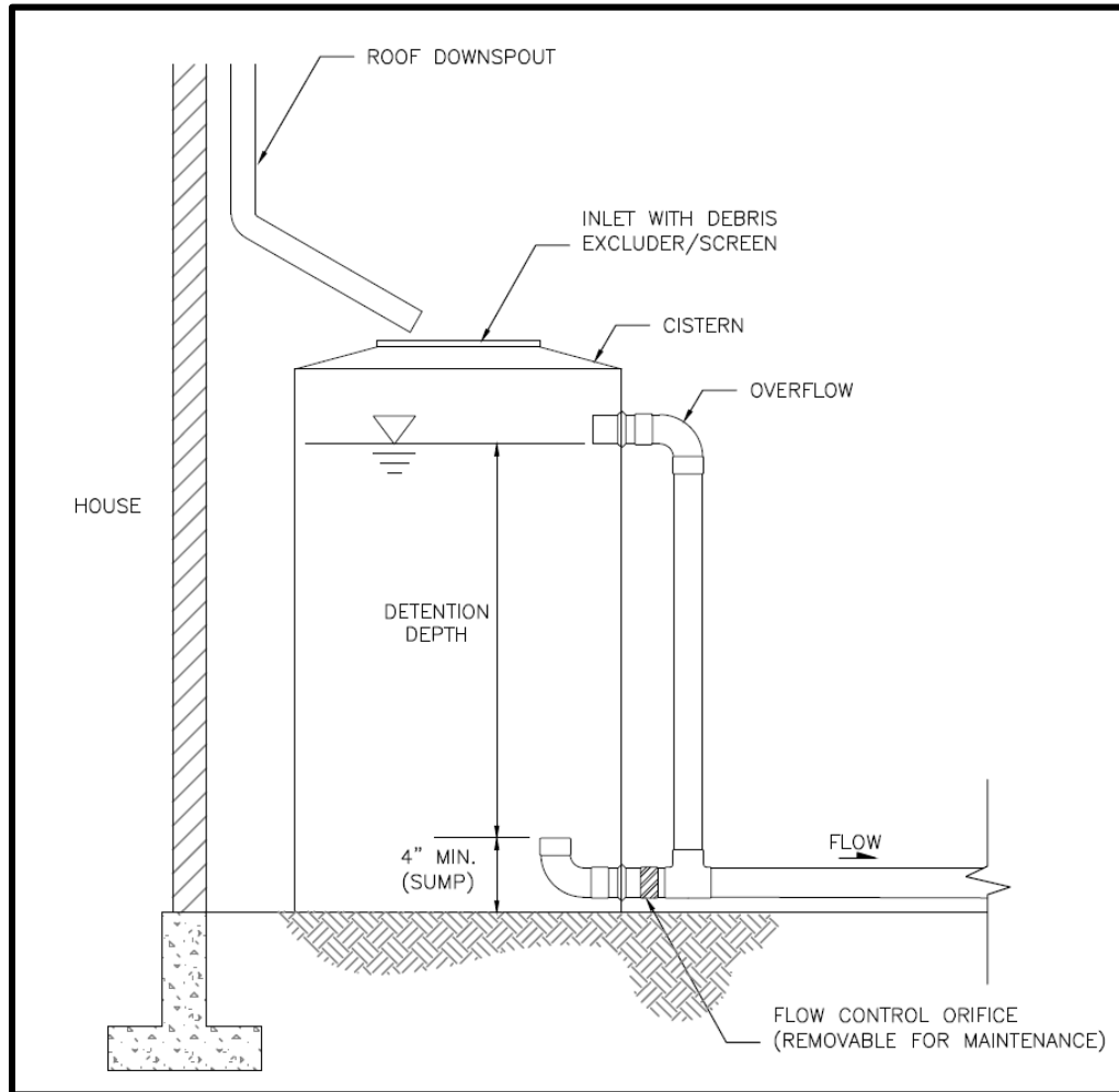
Figure 5.28. Detention Cistern.
