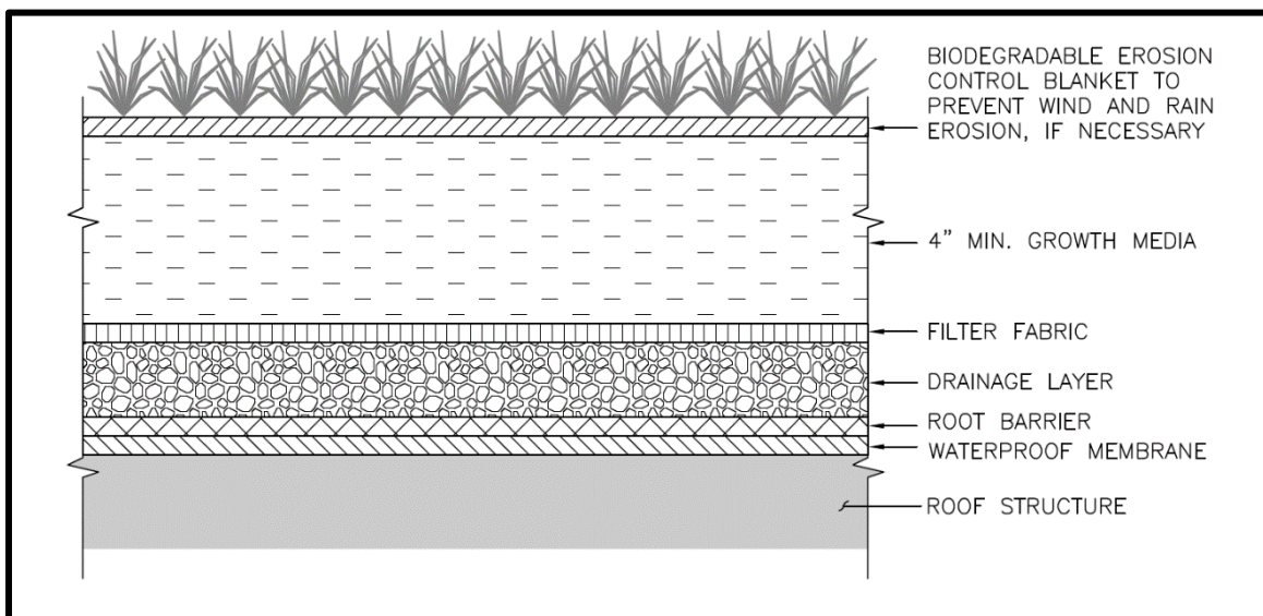
Figure 5.24. Vegetated Roof System.
