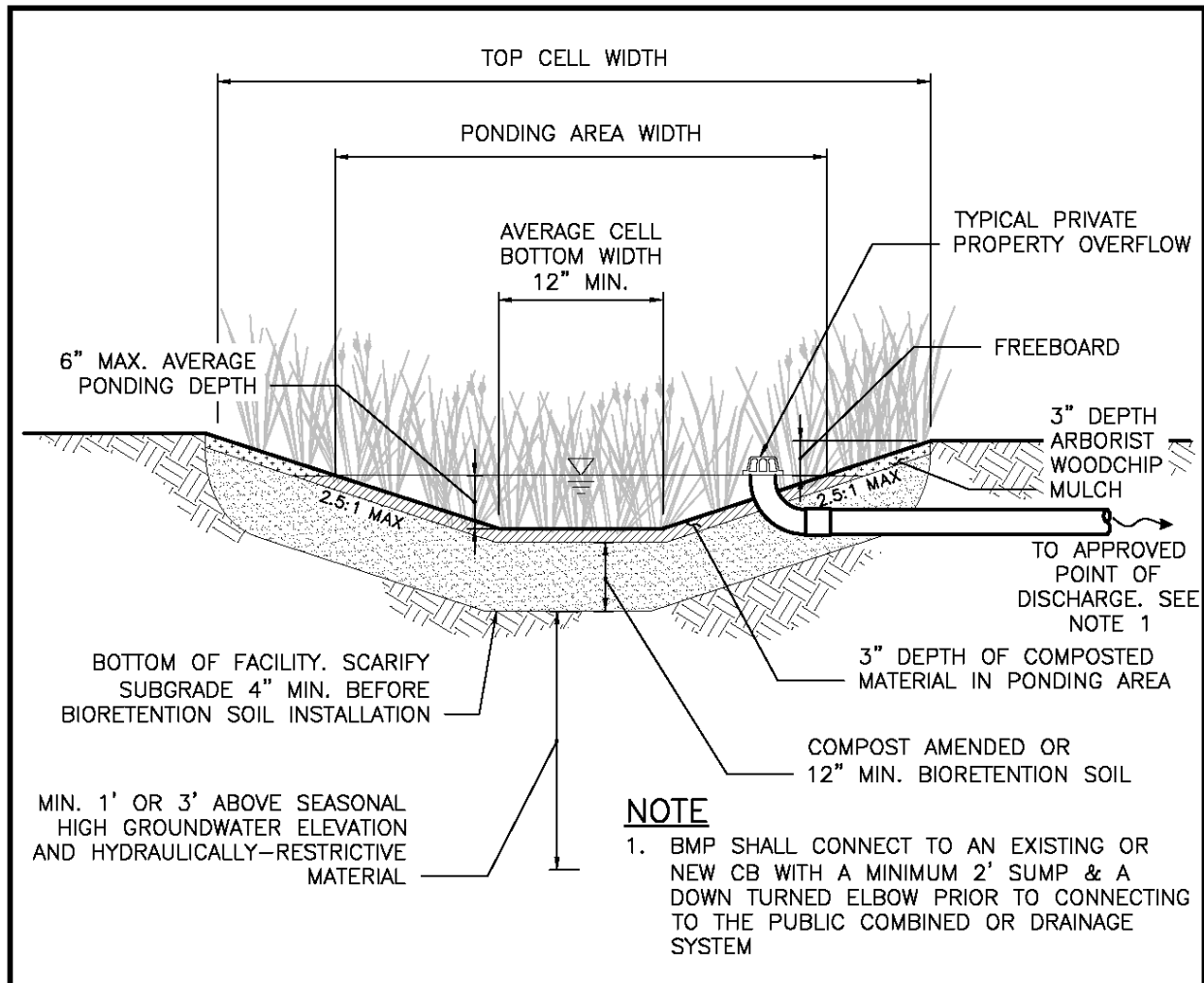
Figure 5.16. Typical Rain Garden.
