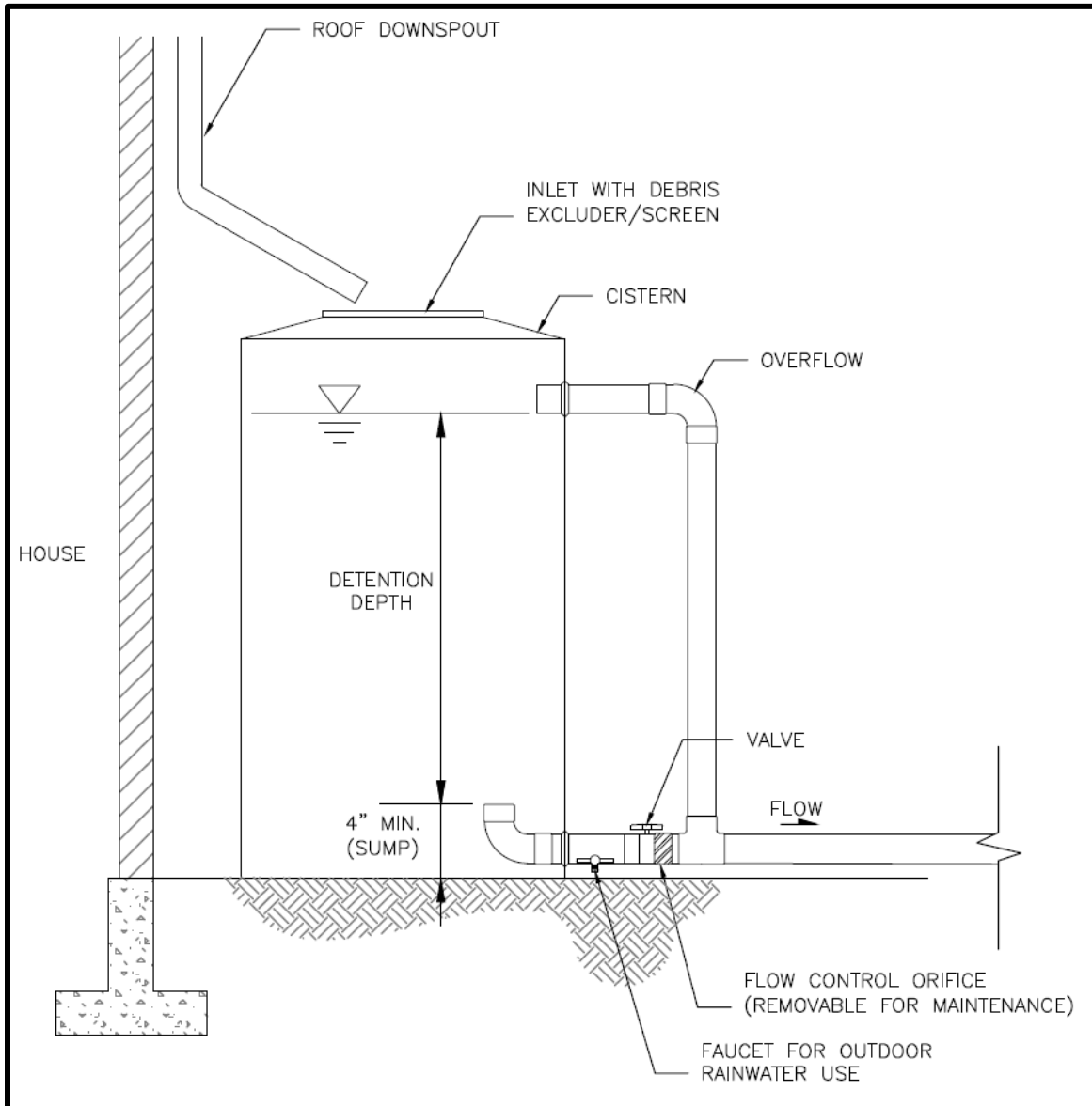
Figure 5.23. Detention Cistern with Harvesting Capacity for Single-Family Residential Projects Only.
