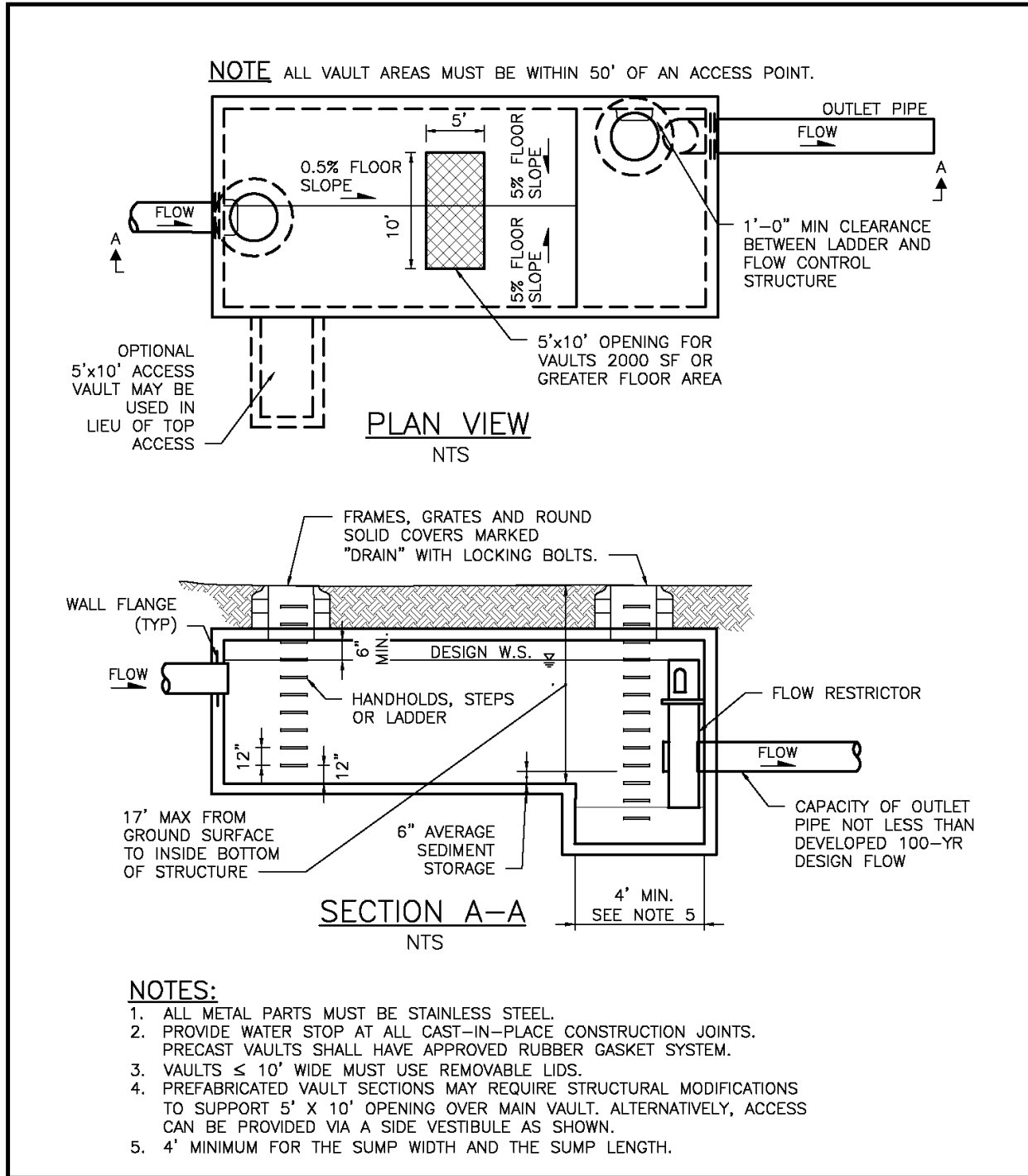
Figure 5.27. Typical Detention Vault.
