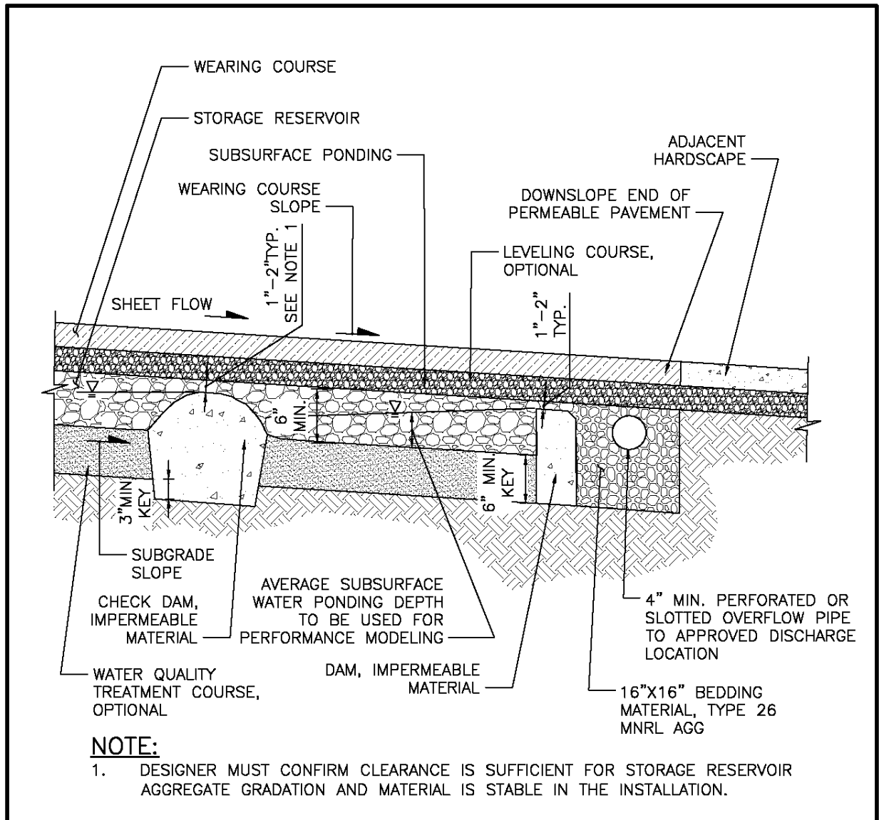
Figure 5.18. Example Permeable Pavement Facility with Checkdams.
