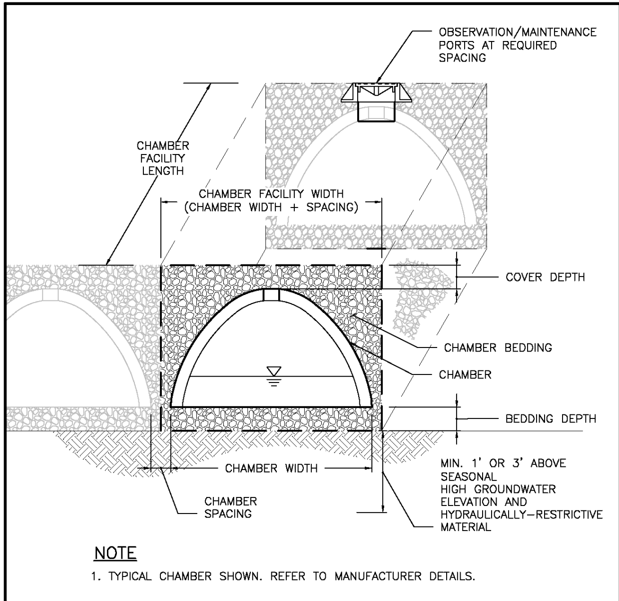
Figure 5.22. Typical Infiltration Chamber/Vault.
