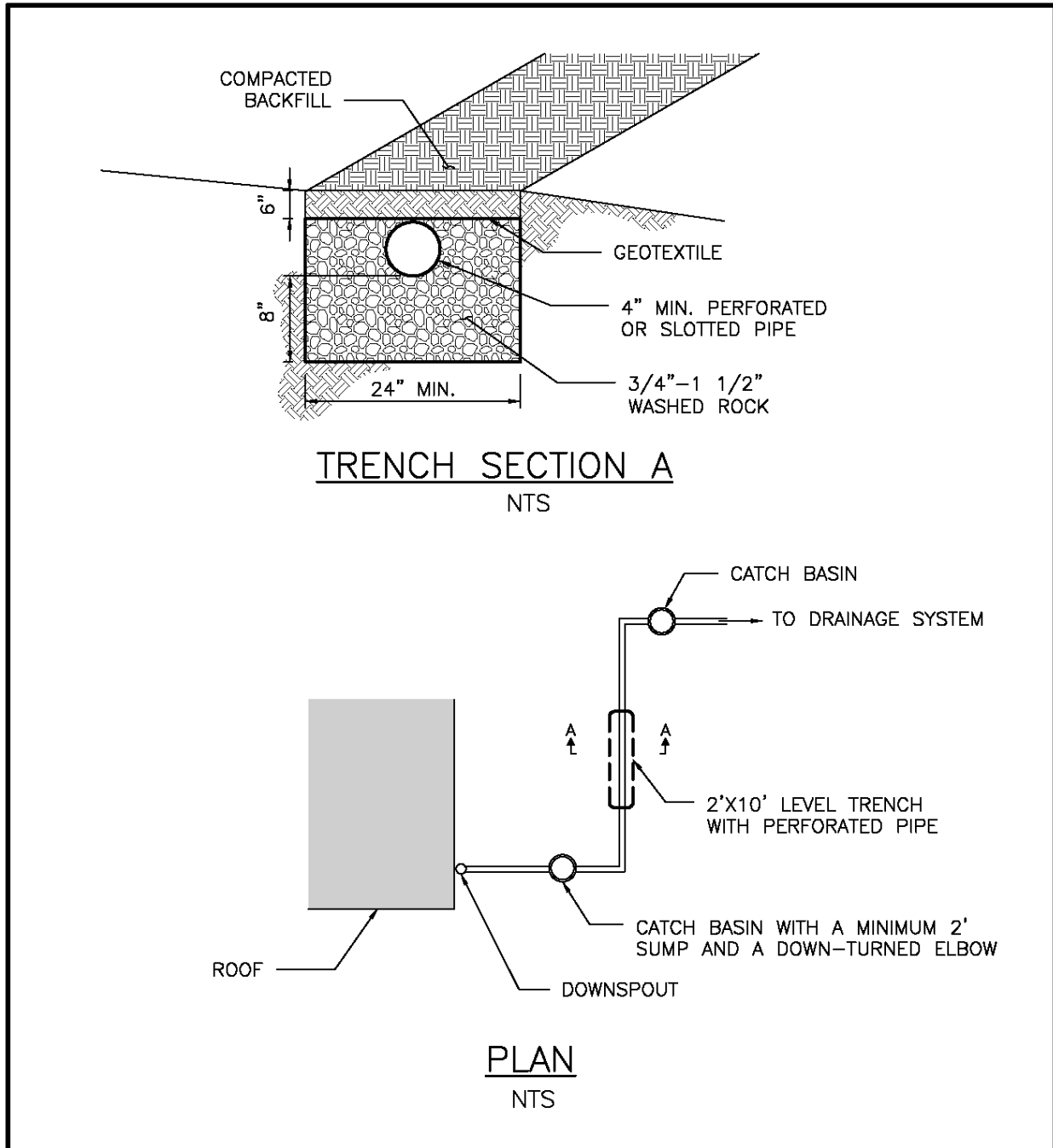
Figure 5.21. Perforated Stub-Out Connection.
