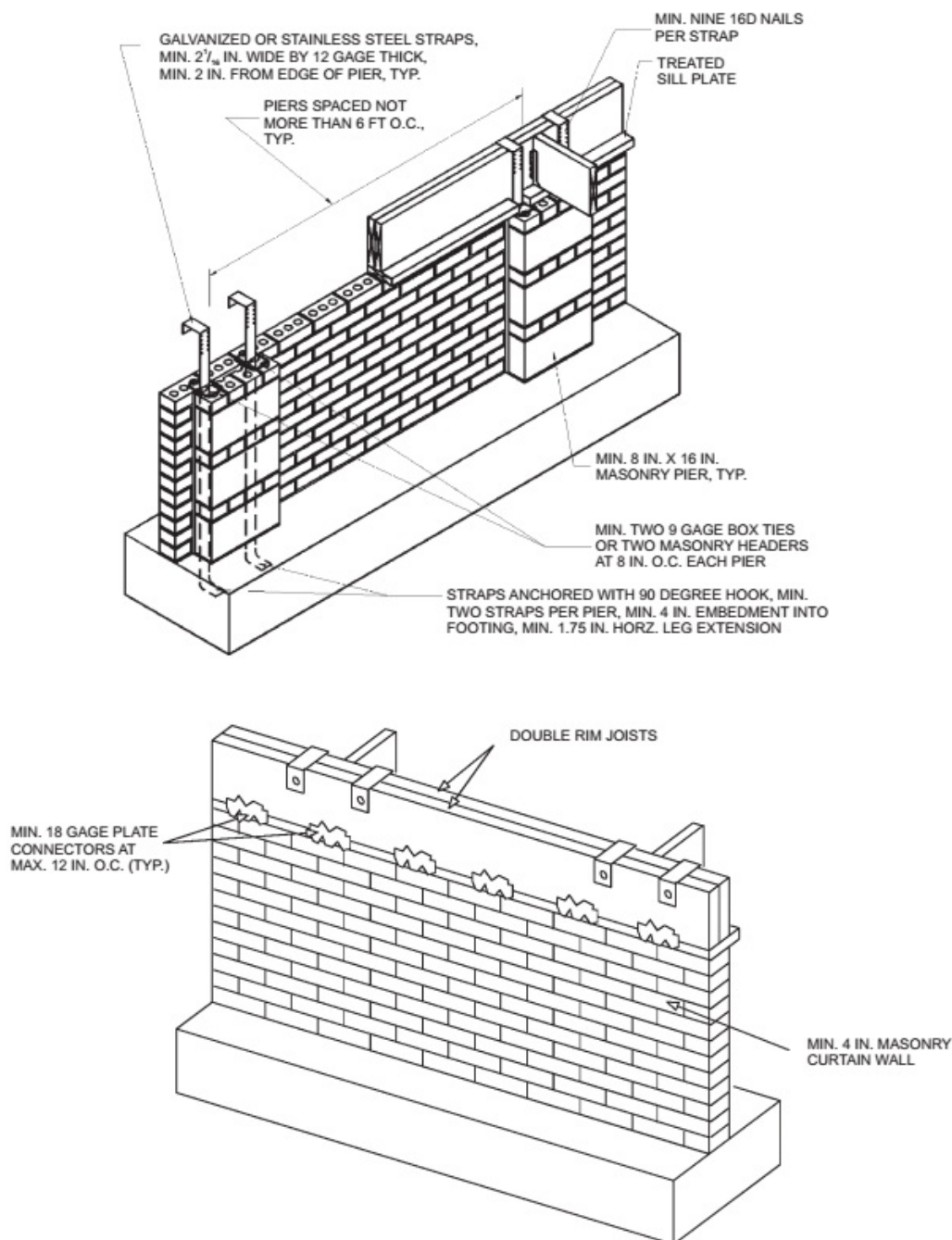
FIGURE R404.1.5.3 FOUNDATION WALL CLAY MASONRY CURTAIN WALL WITH CONCRETE MASONRY PIERS
