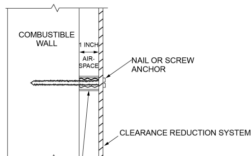
FIGURE G2409.2(1) [308.2(1)] EXTENT OF PROTECTION NECESSARY TO REDUCE CLEARANCES FROM GAS EQUIPMENT OR VENT CONNECTORS
