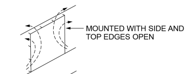
FIGURE G2409.2(1) [308.2(1)] EXTENT OF PROTECTION NECESSARY TO REDUCE CLEARANCES FROM GAS EQUIPMENT OR VENT CONNECTORS
