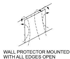
FIGURE G2409.2(1) [308.2(1)] EXTENT OF PROTECTION NECESSARY TO REDUCE CLEARANCES FROM GAS EQUIPMENT OR VENT CONNECTORS
