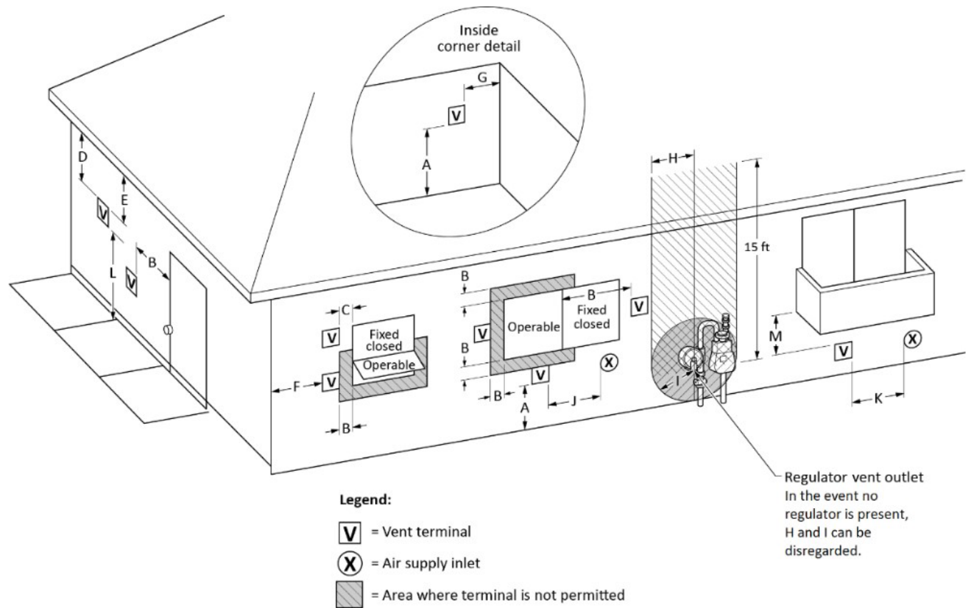
FIGURE G2427.8 (503.8) THROUGH-THE-WALL VENT TERMINAL CLEARANCES
