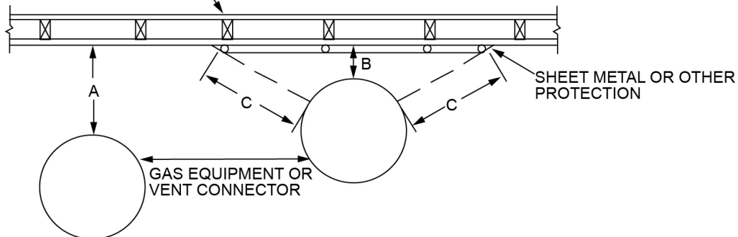
FIGURE G2409.2(1) [308.2(1)] EXTENT OF PROTECTION NECESSARY TO REDUCE CLEARANCES FROM GAS EQUIPMENT OR VENT CONNECTORS
