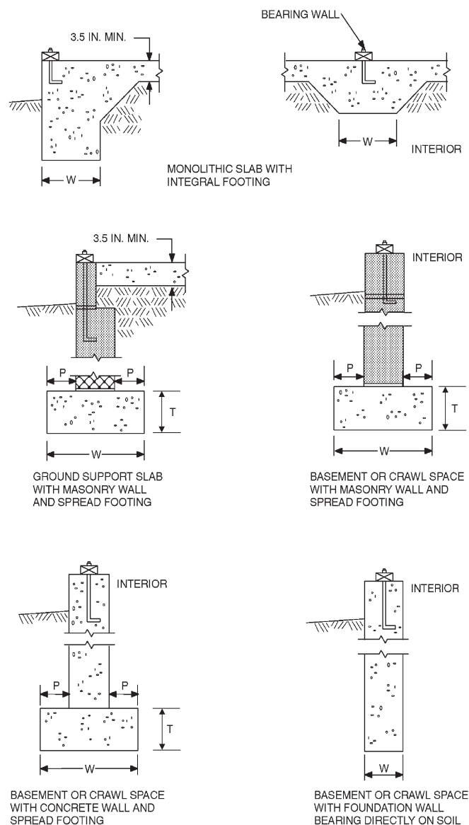
FIGURE R403.1(1) CONCRETE AND MASONRY FOUNDATION DETAILS
