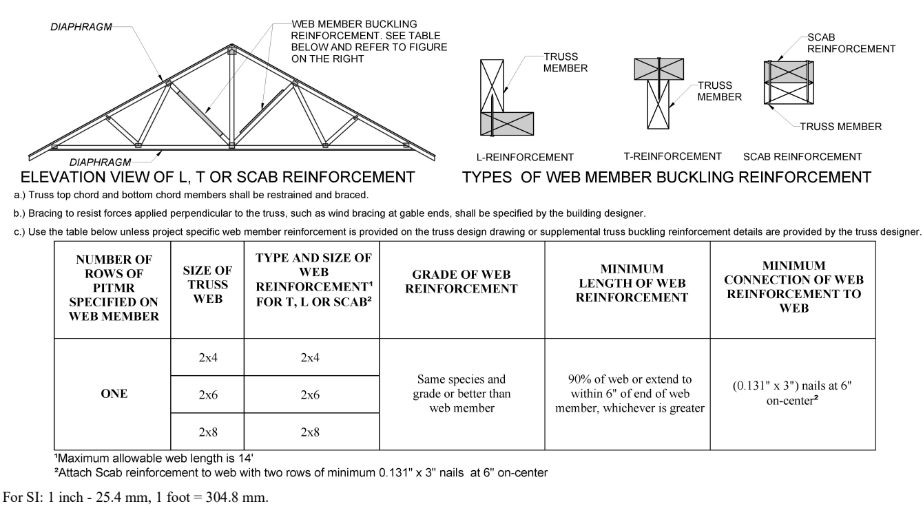
FIGURE 2303.4.1.2(2) ALTERNATIVE INSTALLATION USING BUCKLING REINFORCEMENT FOR TRUSS WEB MEMBERS IN LIEU OF ONE ROW OF PITMR
