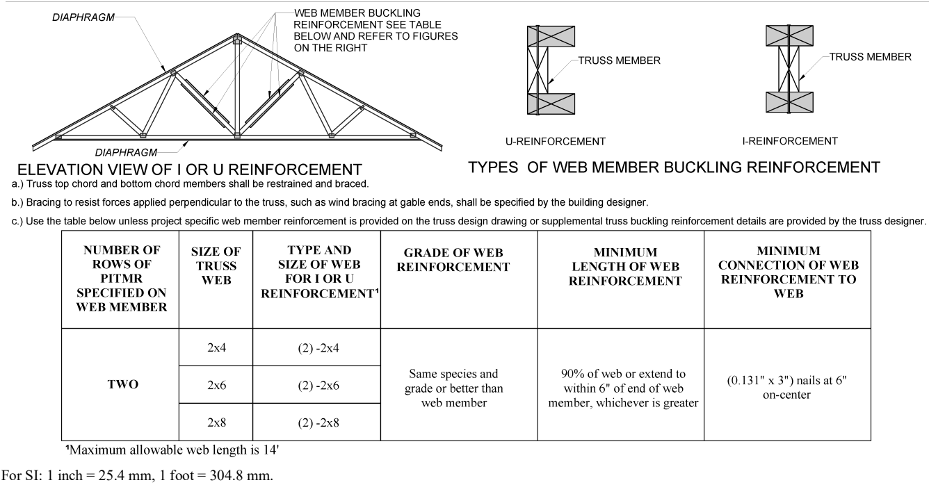
FIGURE 2303.4.1.2(4) ALTERNATIVE INSTALLATION USING BUCKLING REINFORCEMENT FOR TRUSS WEB MEMBERS IN LIEU OF TWO ROWS OF PITMR
