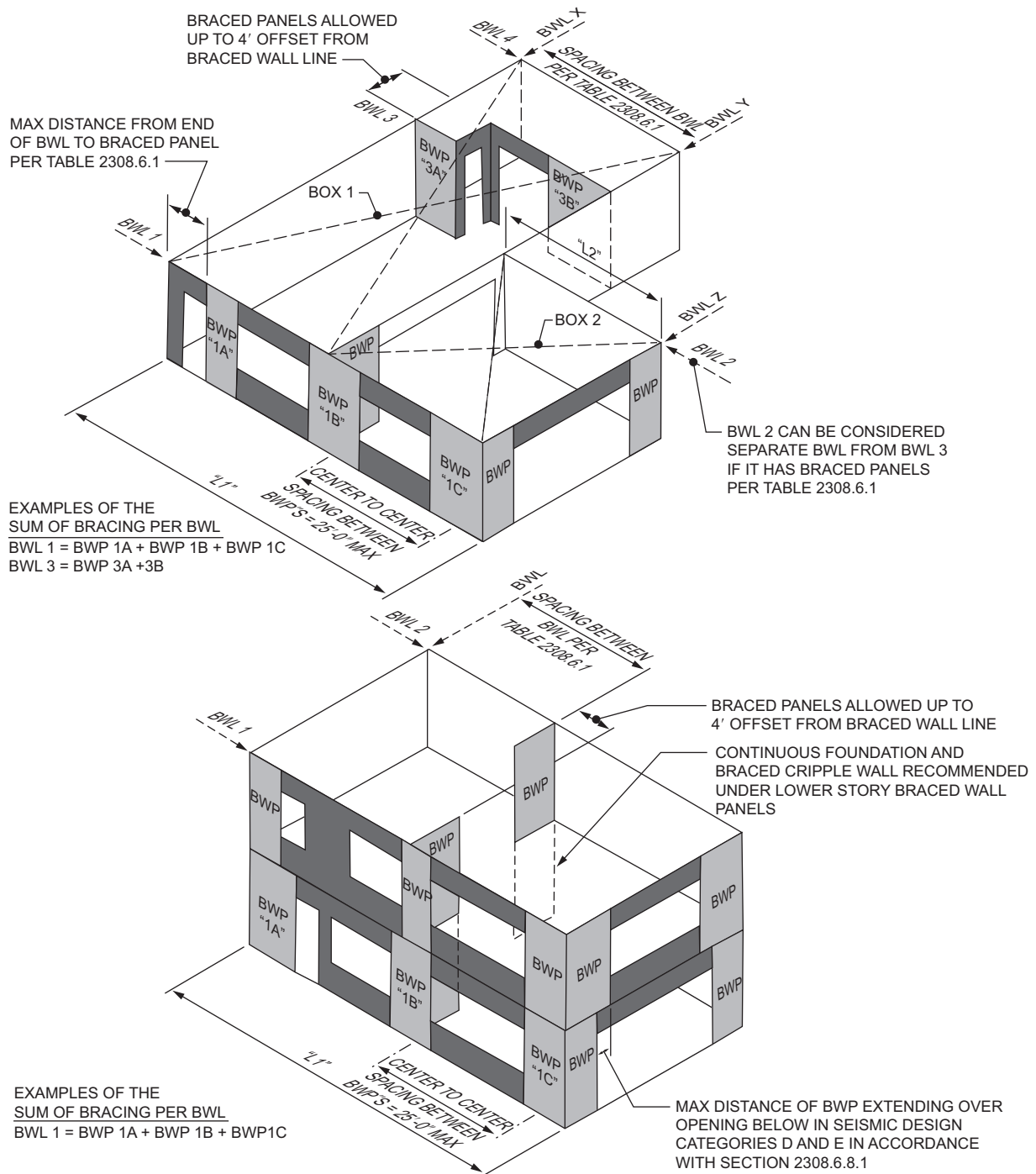
FIGURE 2308.6.1 BASIC COMPONENTS OF THE LATERAL BRACING SYSTEM
