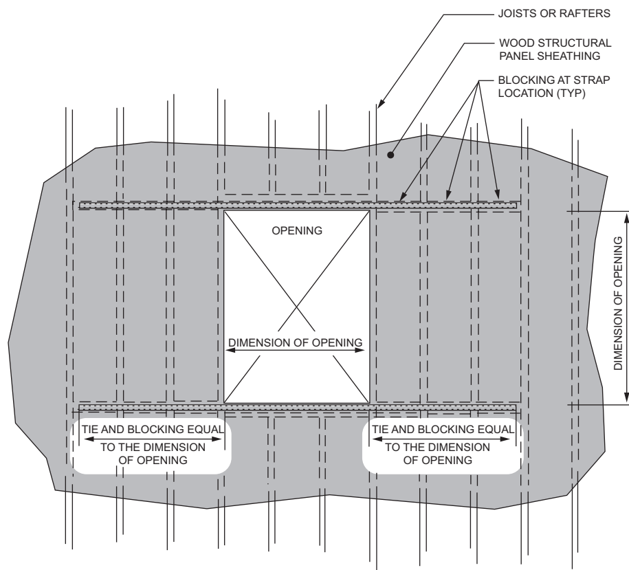
FIGURE 2308.4.4.1(1) OPENINGS IN FLOOR AND ROOF DIAPHRAGMS
