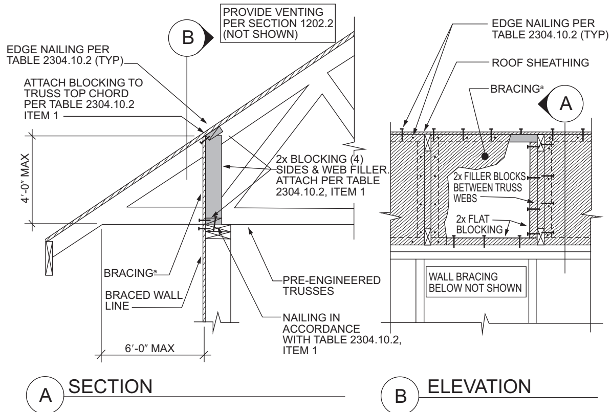
FIGURE 2308.6.7.2(2) BRACED WALL PANEL TOP PLATE CONNECTION
