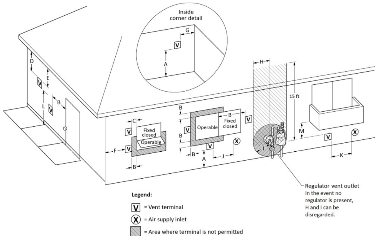
FIGURE 503.8 THROUGH-THE-WALL VENT TERMINAL CLEARANCE
