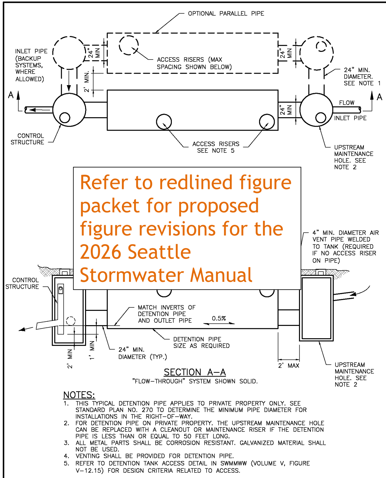
Figure 5.28. Typical Private Property Detention Pipe.
