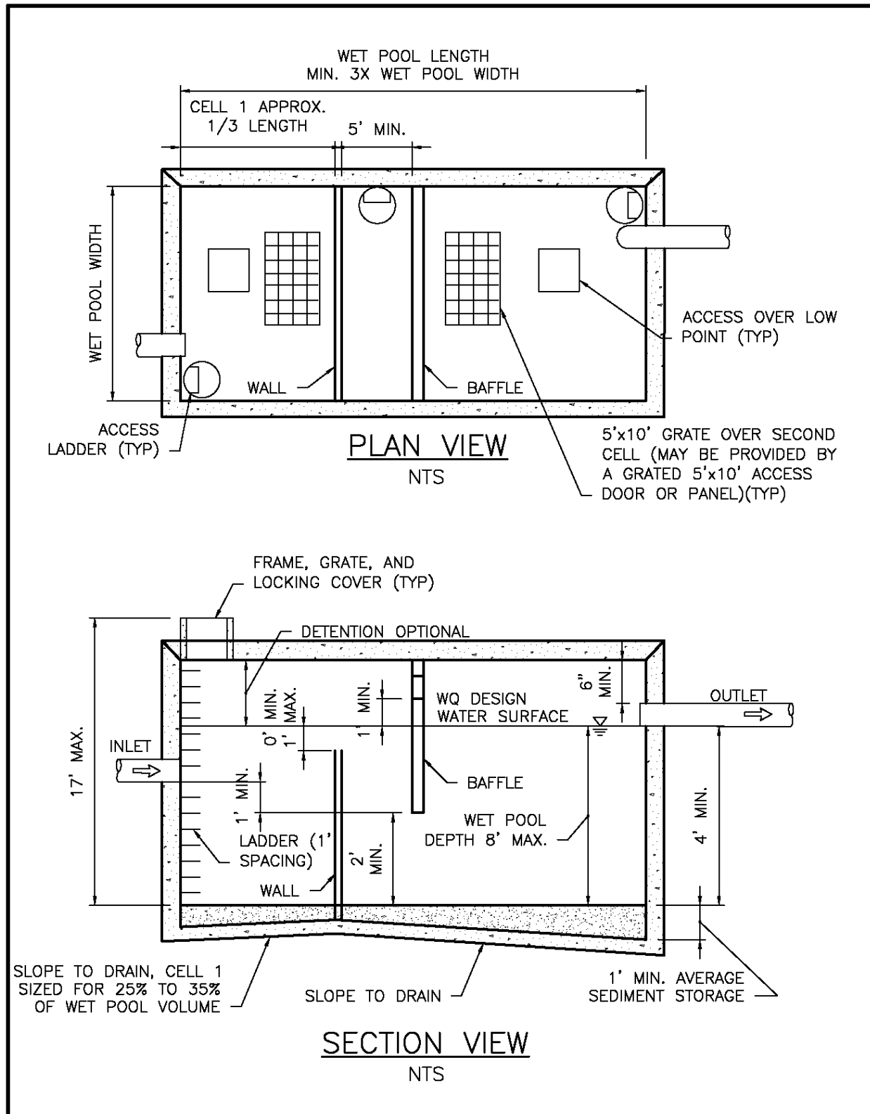
Figure 5.34. Typical Wet Vault.
