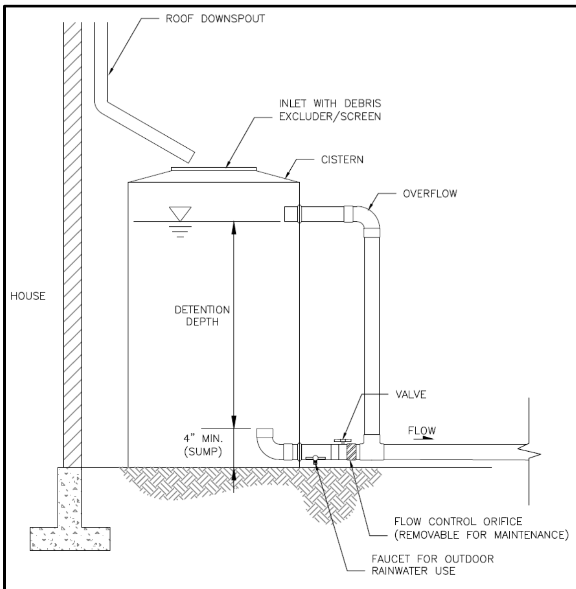
Figure 5.25. Detention Cistern with Harvesting Capacity for Single-Family Residential Projects Only.
