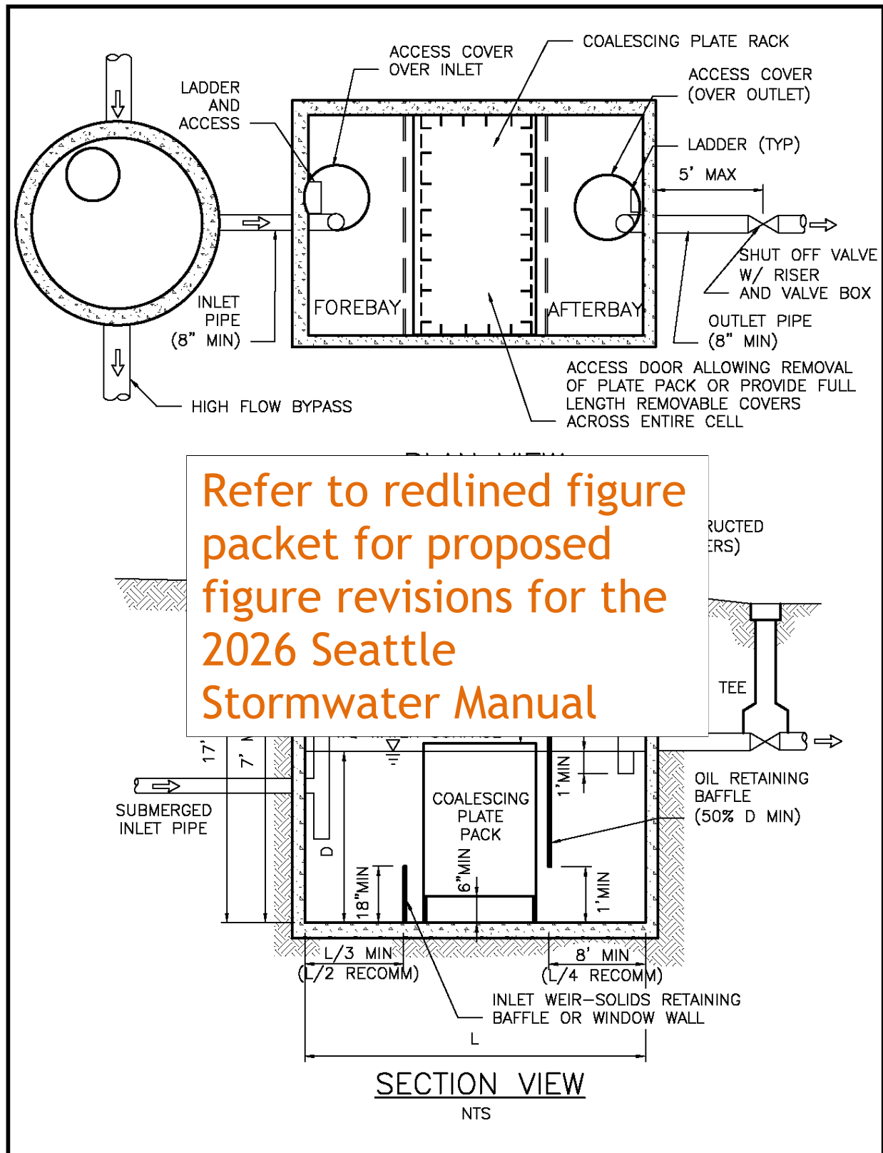
Figure 5.36. Typical Coalescing Plate Separator.
