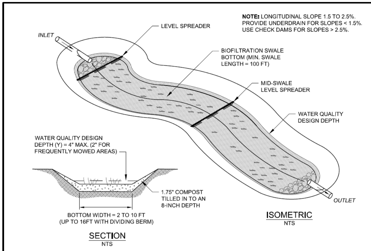
Figure 5.33. Biofiltration Swale Plan and Profile.
