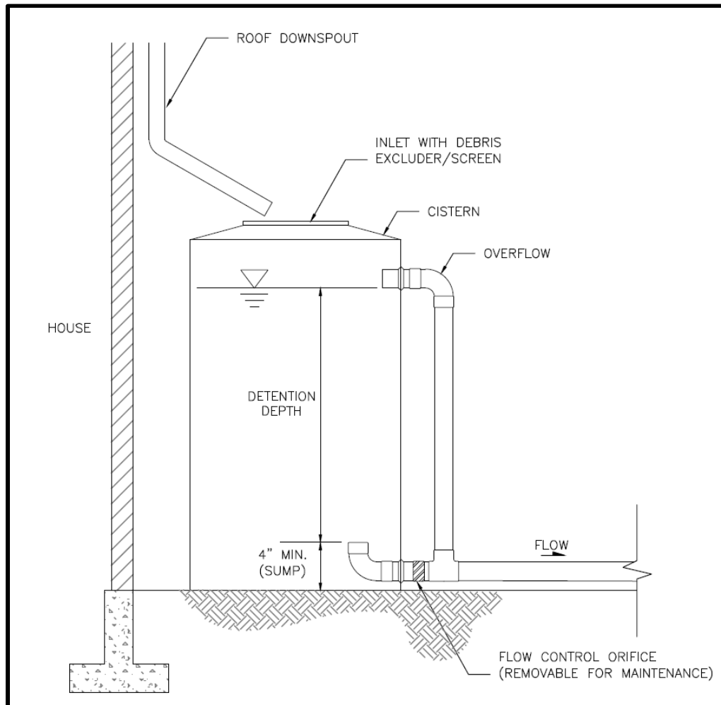
Figure 5.30. Detention Cistern.
