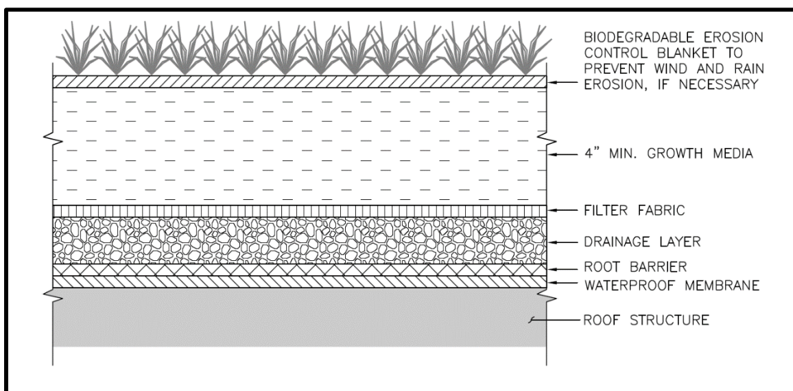
Figure 5.26. Vegetated Roof System.
