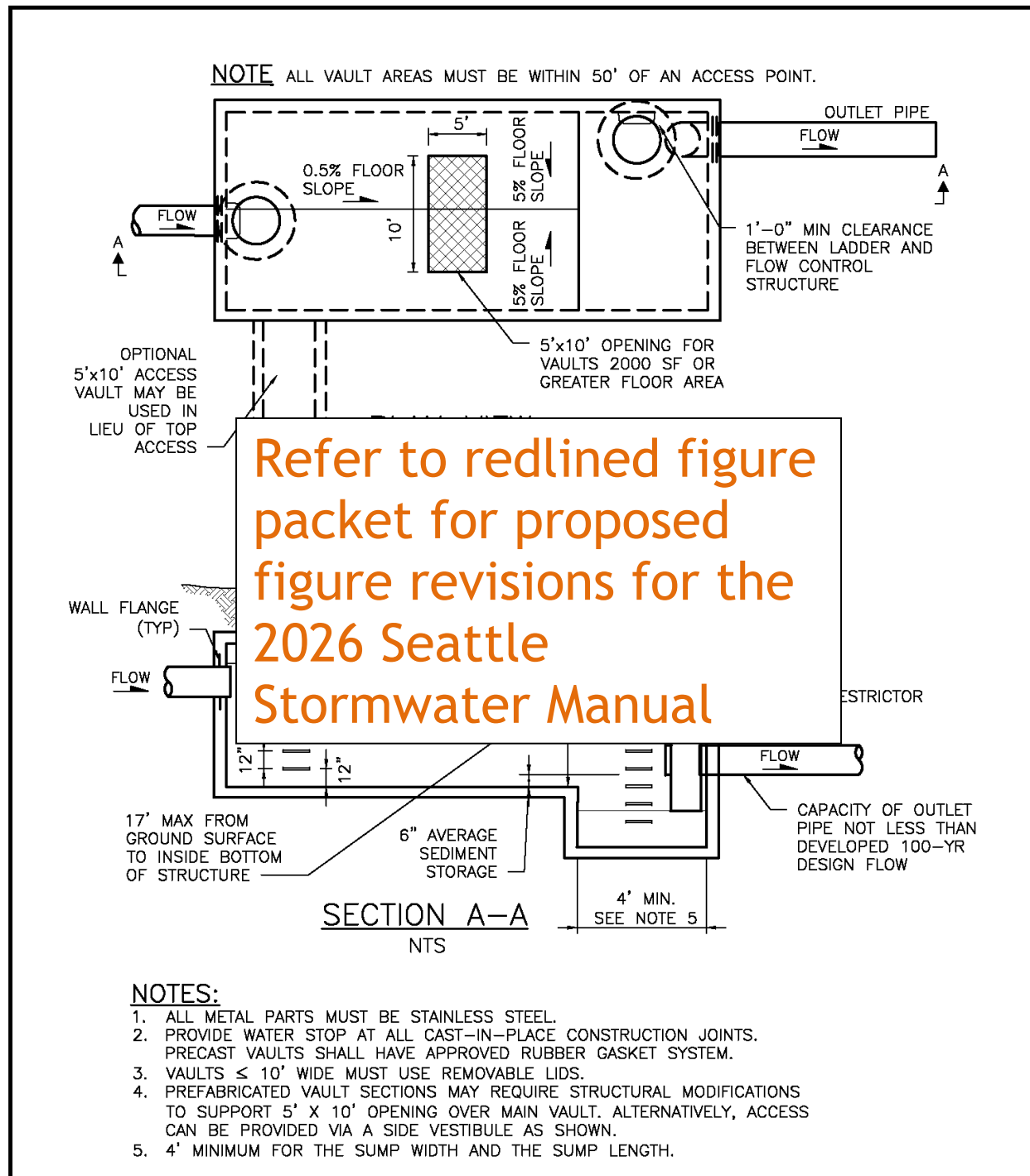
Figure 5.29. Typical Detention Vault.
