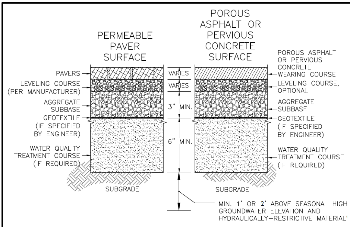
Figure 5.27. Permeable Pavement Surface.
