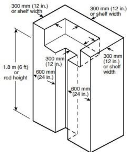
FIGURE 410.2 Closet Storage Space.
