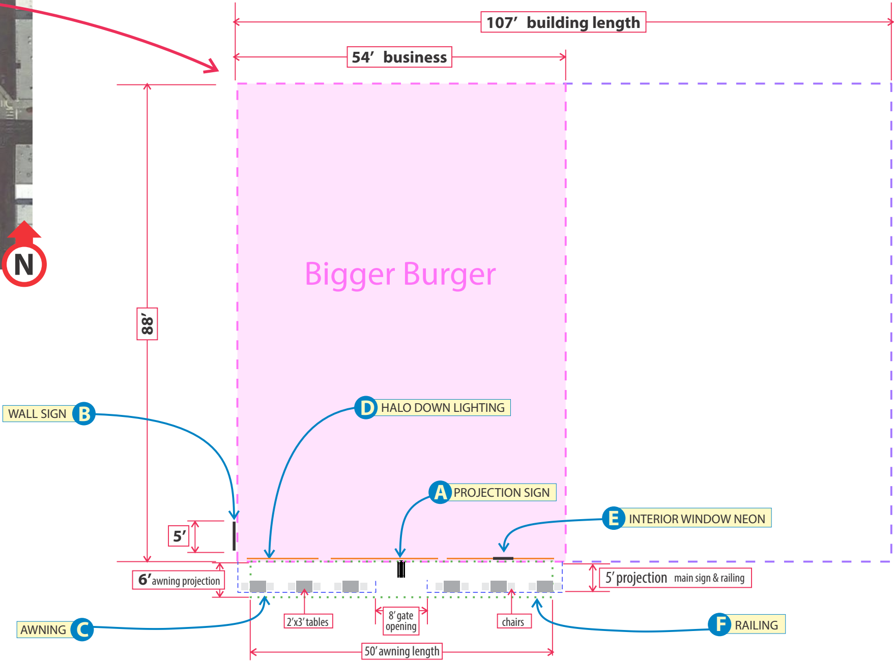
PLOT PLAN DETAIL Scale" 1/16" = 1'
