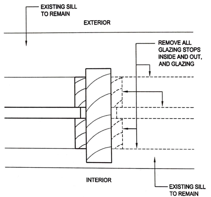
EXISTING WINDOW - JAMB CONDITION
