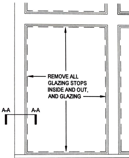
ENLARGED EXISTING WINDOW SCALE: 1/2" = 1'-0"
