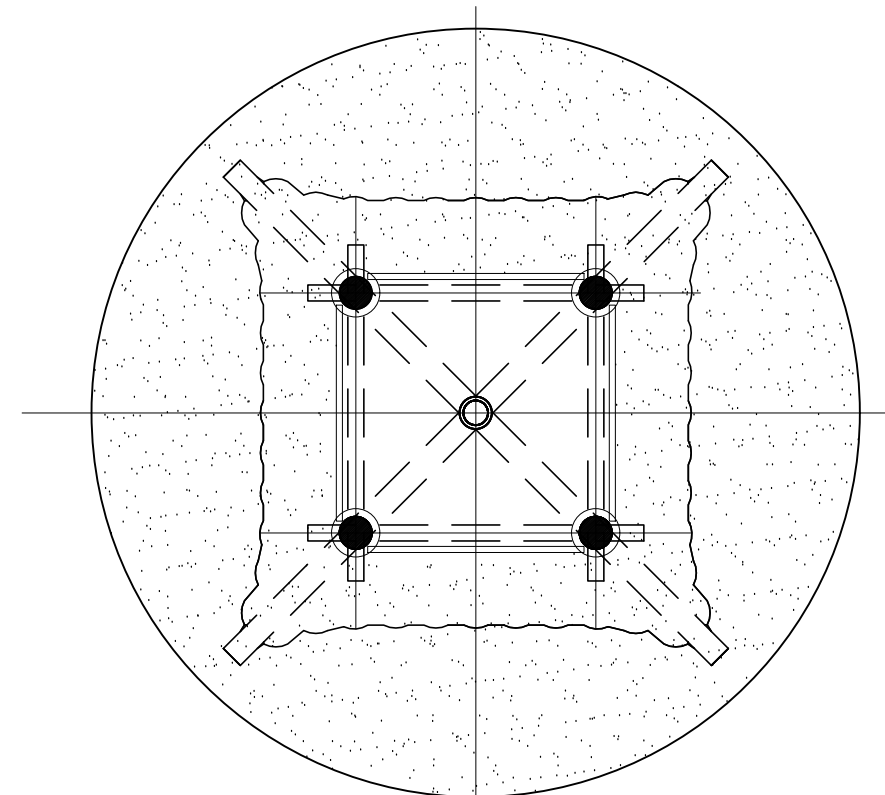
PLAN VIEW SCALE: 1/4" = 1'-0"
