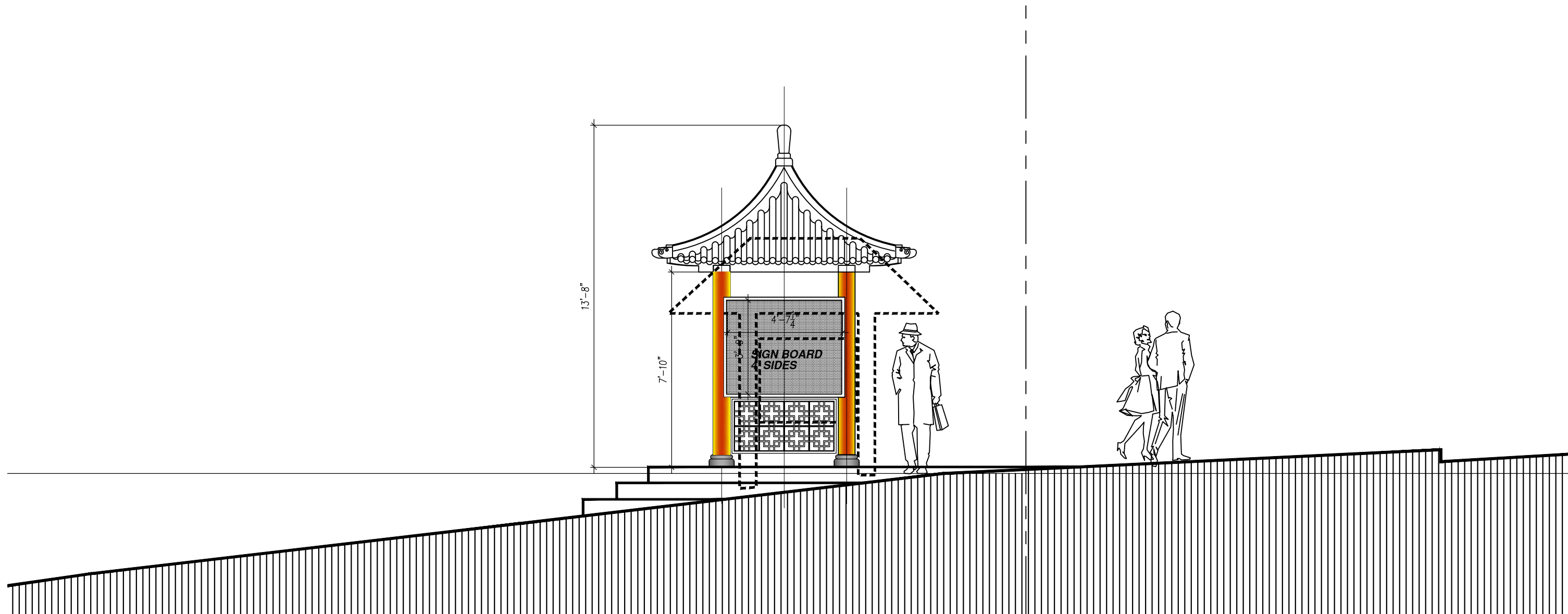
(PARTIAL) SECTION THRU EXST. SIGN MARQUEE
