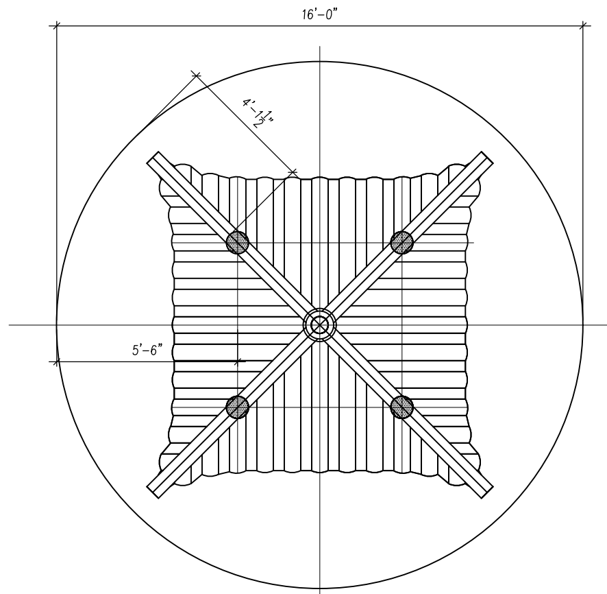
ROOF PLAN SCALE: 1/4" = 1'-0"
