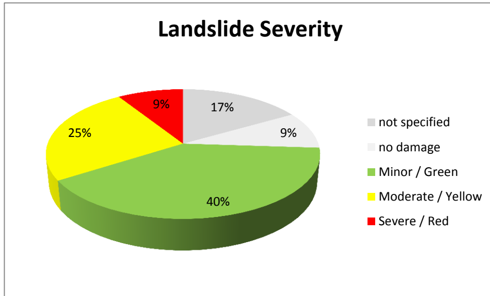
Figure 5. Landslide Severity
