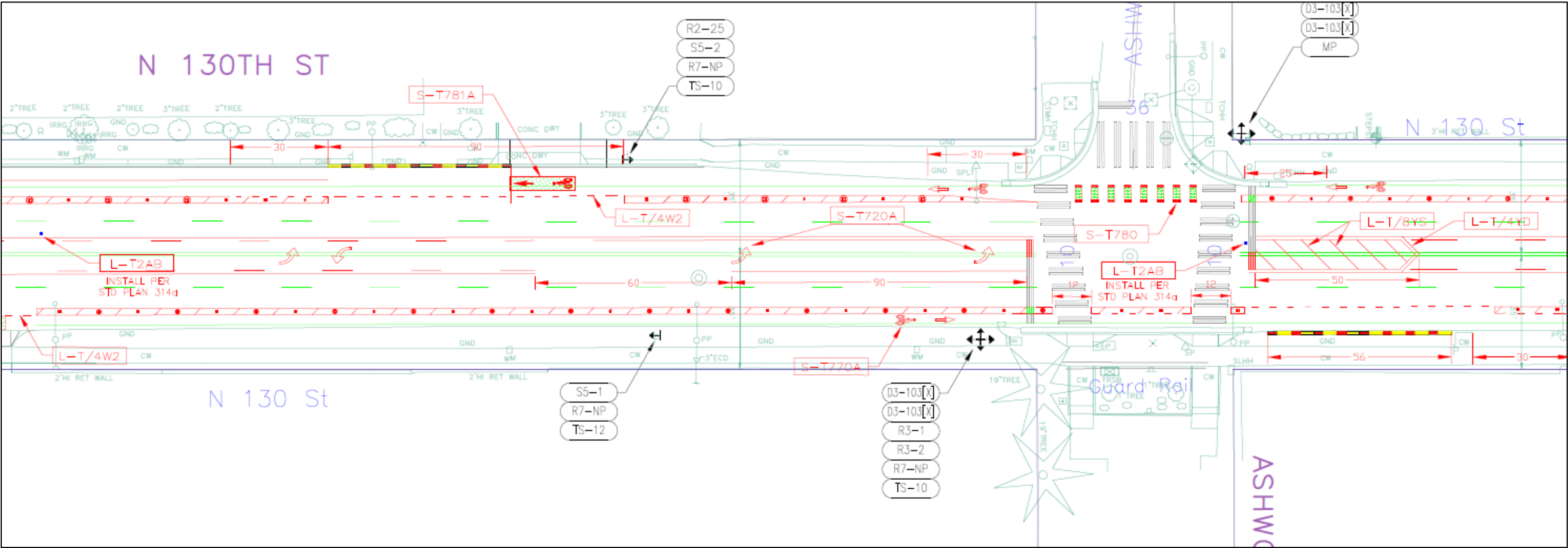
N 130th St Vision Zero Safety Corridor Street redesign layout
