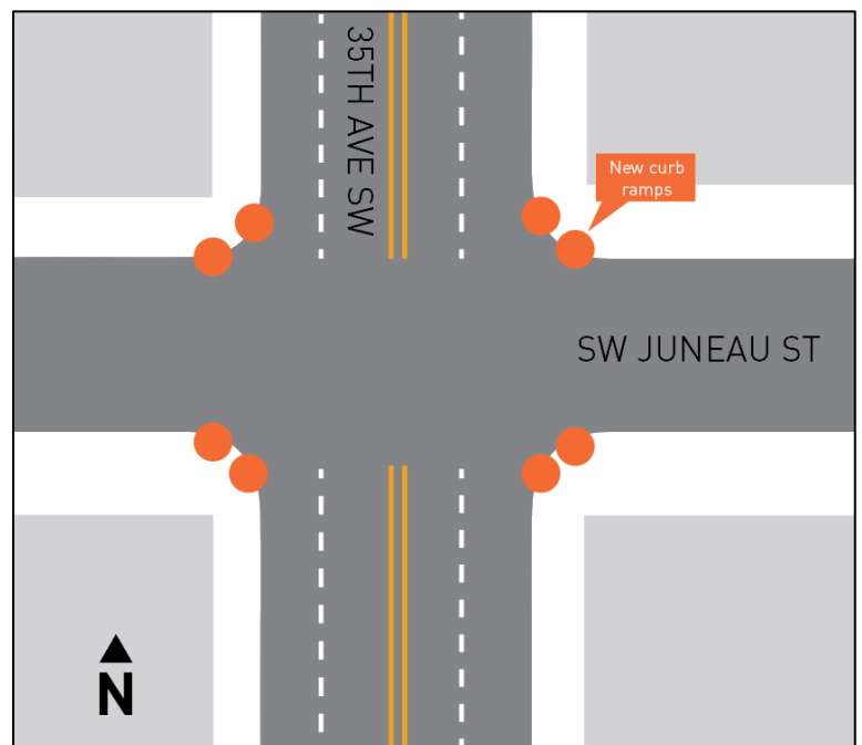
Improvements at 35th Ave SW/SW Juneau St. Image not to scale.
