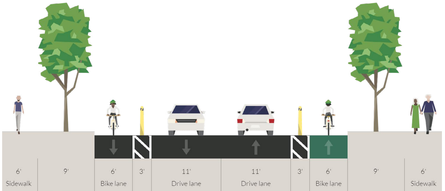
Cross-section view of the S Columbian Way/S Alaska St after paving.
