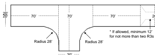
Acceptable Alternative to 120 Foot Hammerhead
