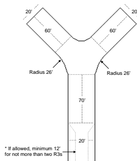
60 Foot Y – Acceptable Alternative to 120 Foot Hammerhead
