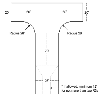
120 Foot Hammerhead
