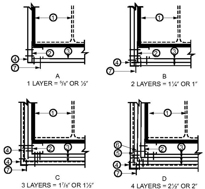
FIGURE 722.5.1(3) GYPSUM-PROTECTED STRUCTURAL STEEL COLUMNS WITH STEEL STUD/SCREW ATTACHMENT SYSTEM
