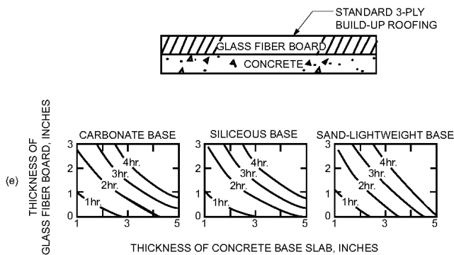
FIGURE 722.2.2.3(2) FIRE-RESISTANCE RATINGS FOR CONCRETE ROOF ASSEMBLIES
