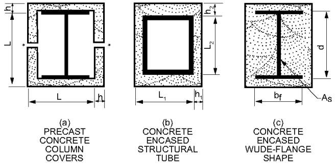
FIGURE 722.5.1(6) CONCRETE PROTECTED STRUCTURAL STEEL COLUMNS a,b
