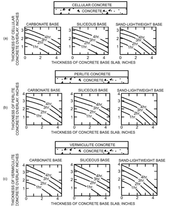
FIGURE 722.2.2.3(1) FIRE-RESISTANCE RATINGS FOR CONCRETE ROOF ASSEMBLIES
