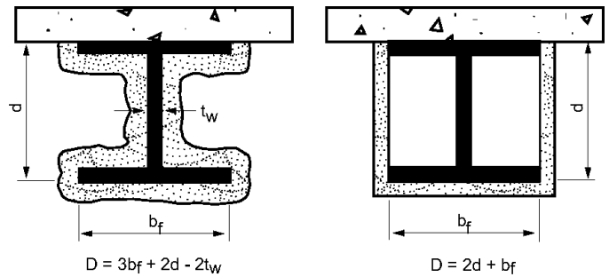
FIGURE 722.5.2 DETERMINATION OF THE HEATED PERIMETER OF STRUCTURAL STEEL BEAMS AND GIRDEES
