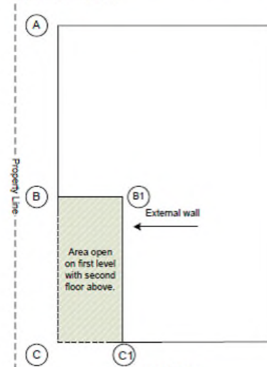
Figure I705.8a Plan View
