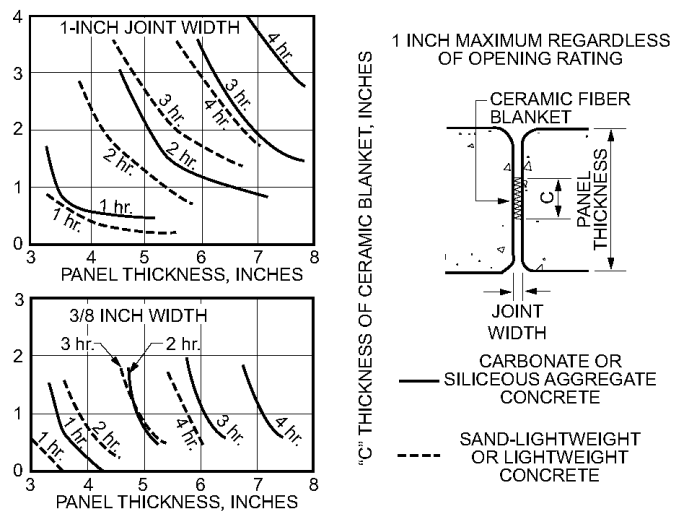
FIGURE 722.2.1.3.1 CERAMIC FIBER JOINT PROTECTION
