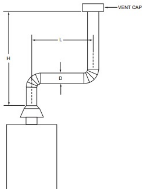
FIGURE B101.4(5) ASBESTOS CEMENT TYPE B OR SINGLE-WALL METAL VENT SYSTEM SERVING A SINGLE DRAFT-HOOD-EQUIPPED APPLIANCE
