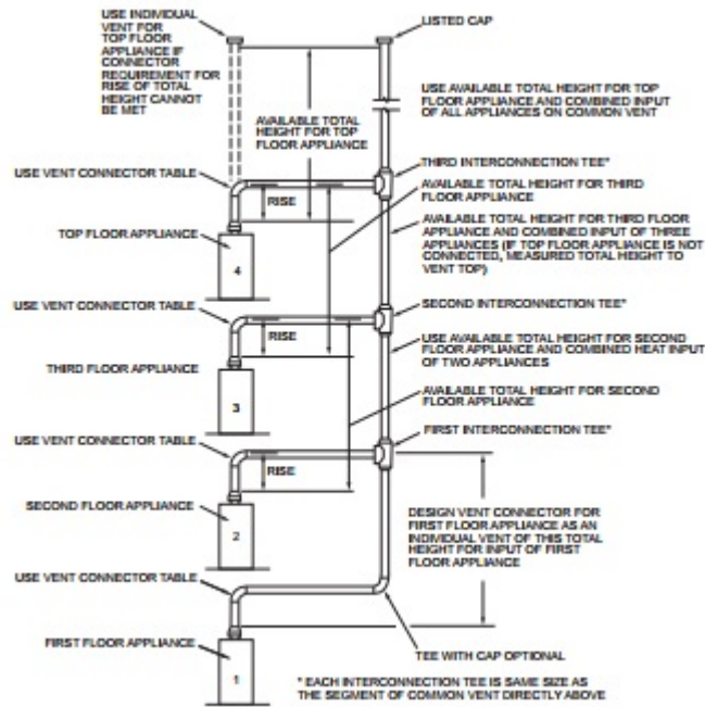
FIGURE B102.5(9) MULTISTORY VENT SYSTEMS
