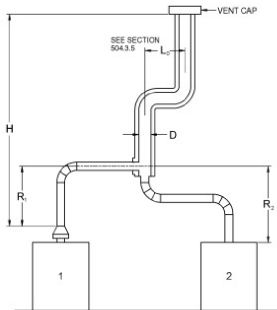
FIGURE B102.5(5) ASBESTOS CEMENT TYPE B OR SINGLE-WALL METAL VENT SYSTEM SERVING TWO OR MORE DRAFT-HOOD-EQUIPPED APPLIANCES
