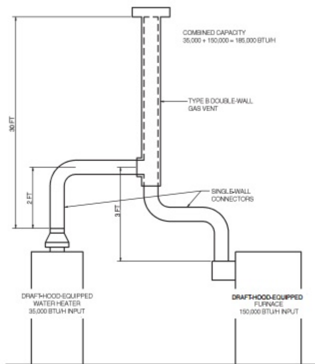
FIGURE B102.1 EXAMPLE 4—COMMON VENTING TWO DRAFT-HOOD-EQUIPPED APPLIANCES
