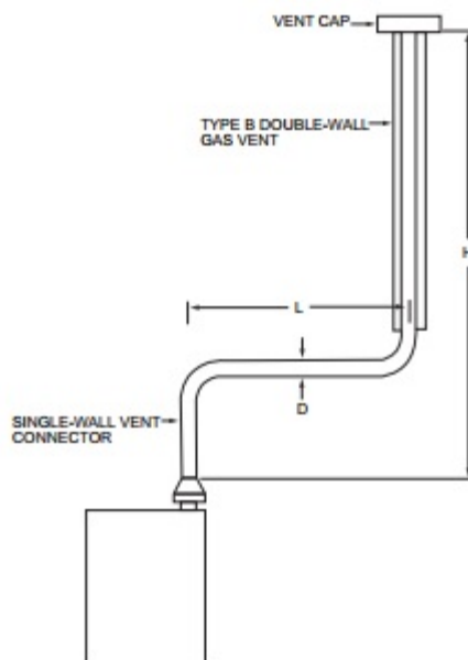
FIGURE B101.4(1) TYPE B DOUBLE-WALL VENT SYSTEM SERVING A SINGLE APPLIANCE WITH A TYPE B DOUBLE-WALL VENT
