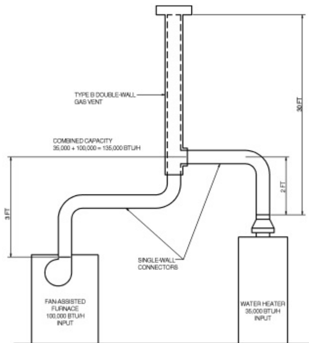
FIGURE B102.2 EXAMPLE 5A—COMMON VENTING A DRAFT HOOD WITH A FAN-ASSISTED FURNACE INTO A TYPE B DOUBLE-WALL COMMON VENT
