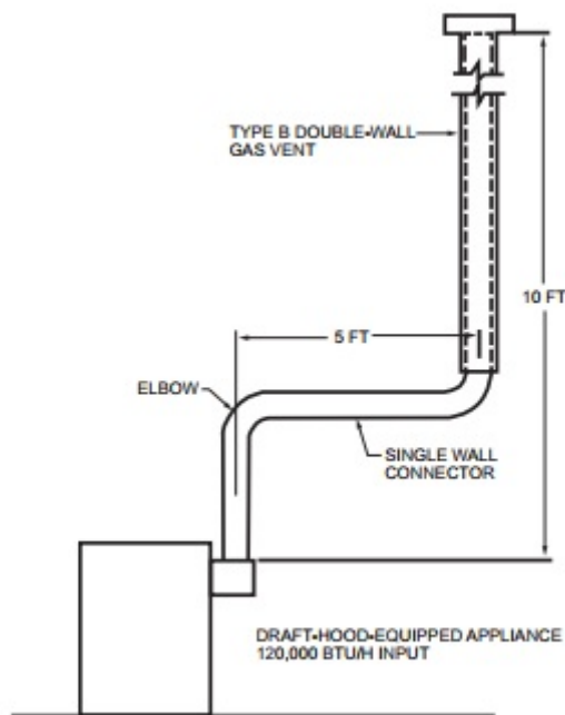
FIGURE B101.1 EXAMPLE 1—SINGLE DRAFT-HOOD-EQUIPPED APPLIANCE
