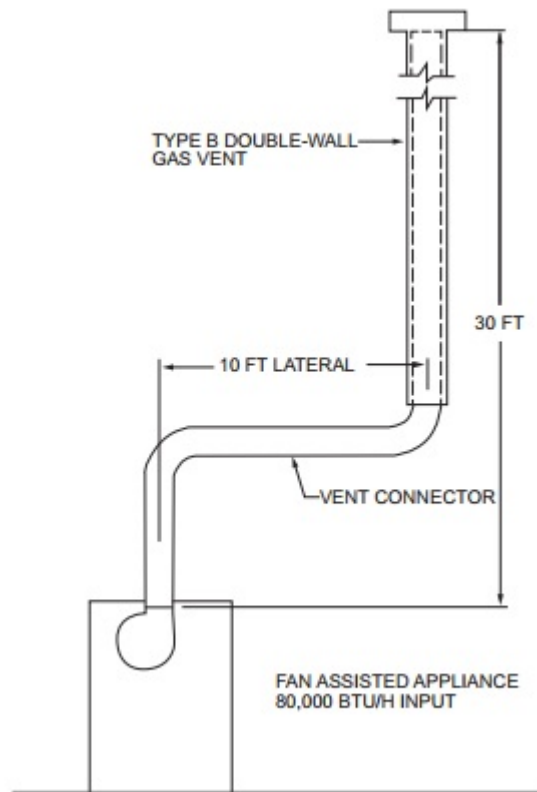
FIGURE B101.2 EXAMPLE 2—SINGLE FAN-ASSISTED APPLIANCE
