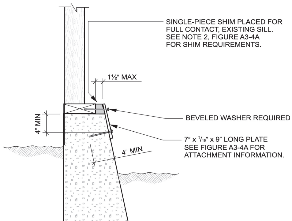
[B] FIGURE A3-4C SILL PLATE ANCHORING TO EXISTING FOUNDATION—ALTERNATE CONNECTION FOR BATTERED FOOTING
