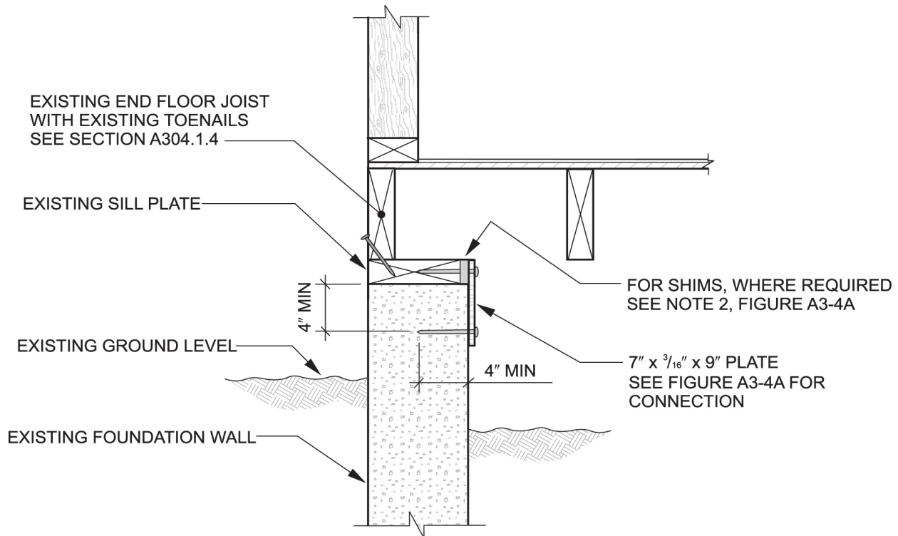
[B] FIGURE A3-4B ALTERNATE SILL PLATE ANCHOR TO EXISTING FOUNDATION WITHOUT CRIPPLE WALL AND FLOOR FRAMING PARALLEL TO FOUNDATIONS
