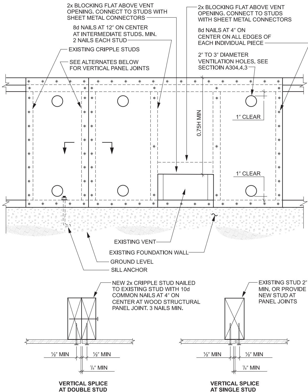
[B] FIGURE A3-7 PARTIAL CRIPPLE STUD WALL ELEVATION
