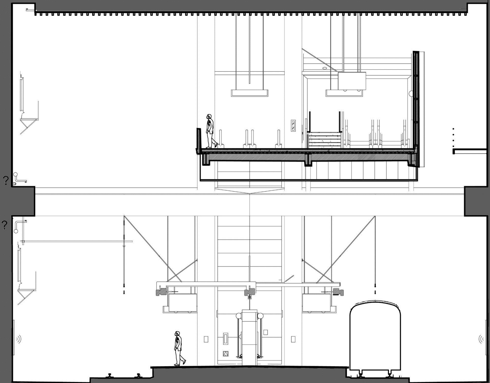
sprinklers + pipes
