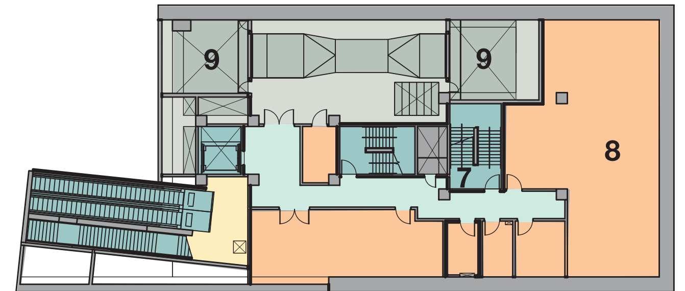
Basement 1 Level
