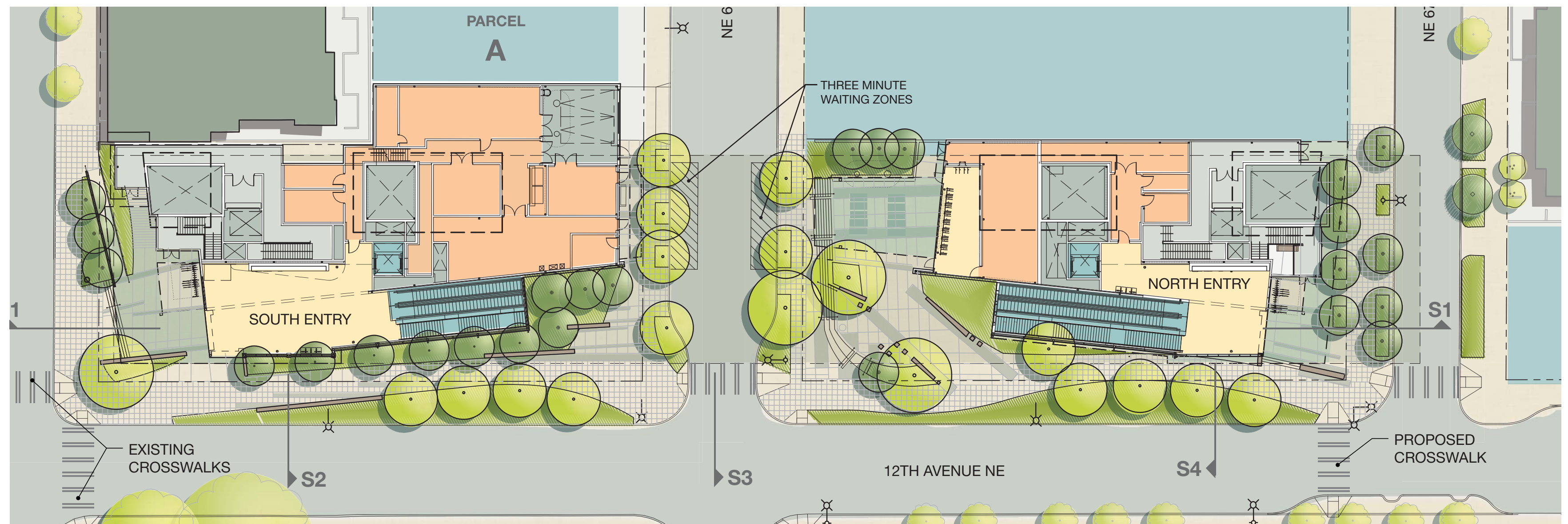
Current Plan
