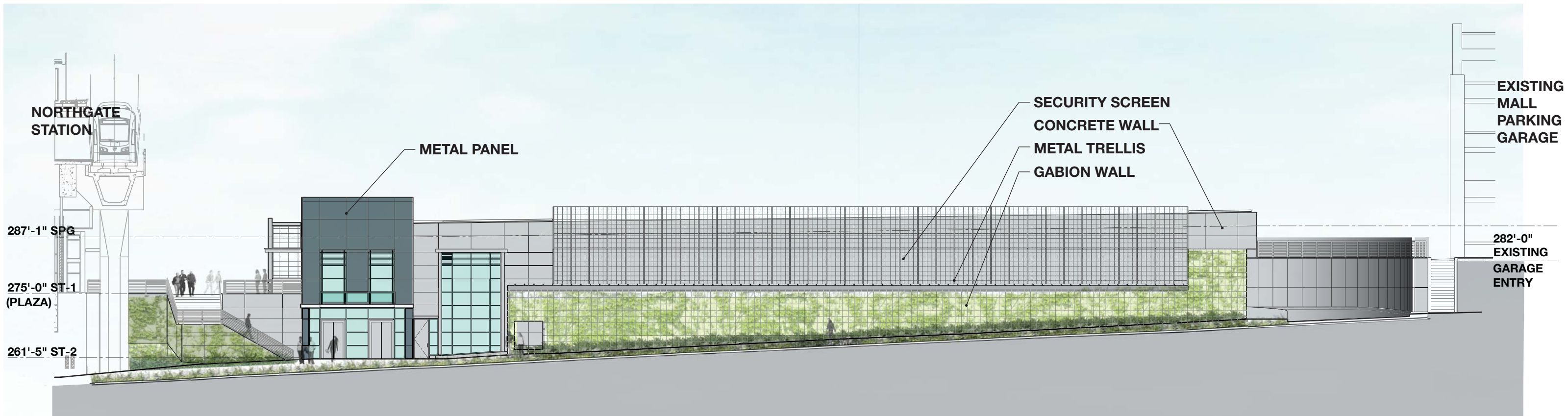
SOUTH ELEVATION - Looking from NE 103RD ST
