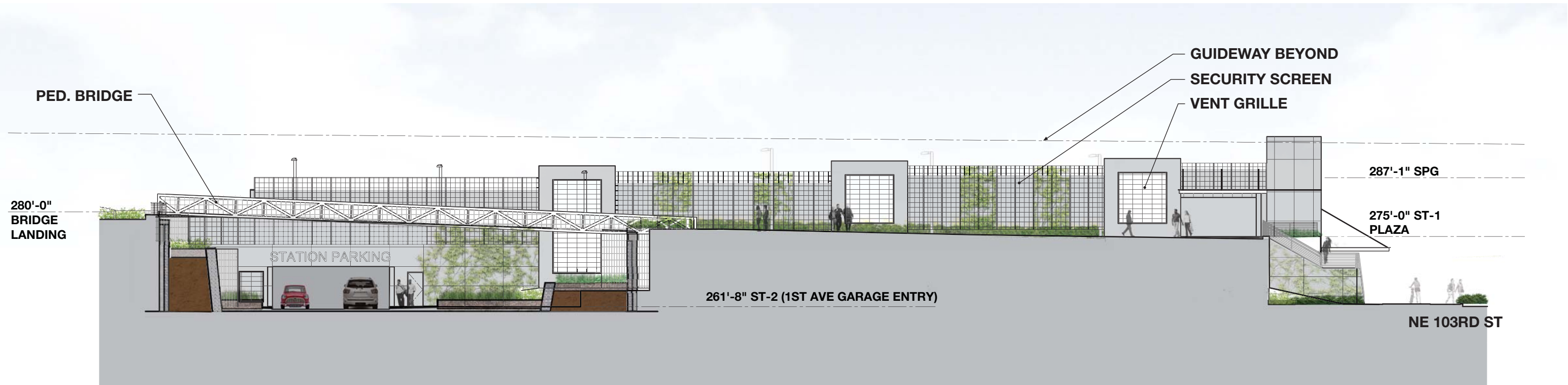
WEST ELEVATION - Looking from Plaza
