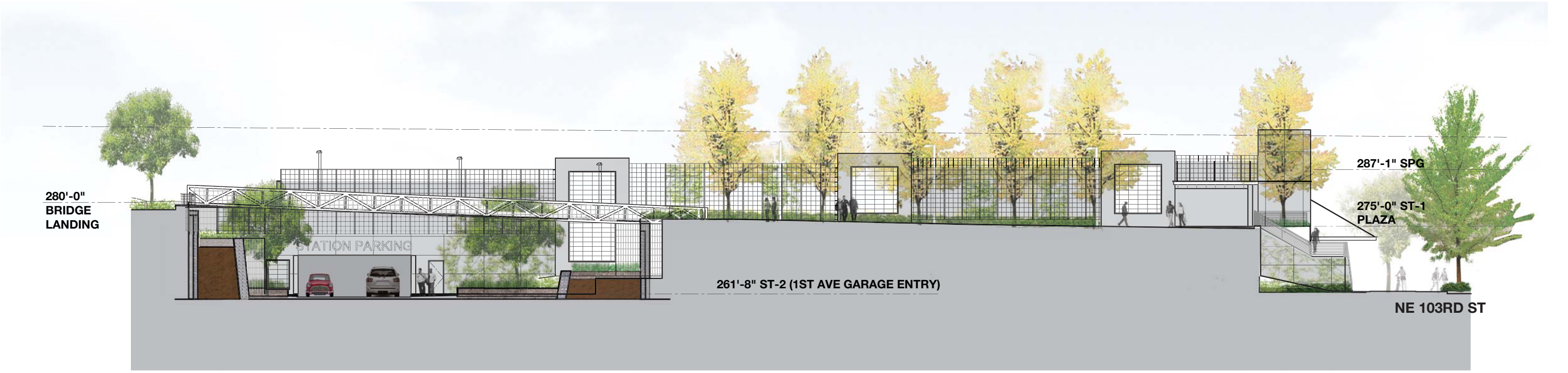
WEST ELEVATION - Looking from Plaza
