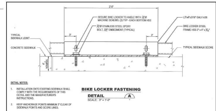
Figure 3.2: Diagram showing the bike locker installation method.
