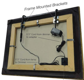
Recommended Dimmer Installation
