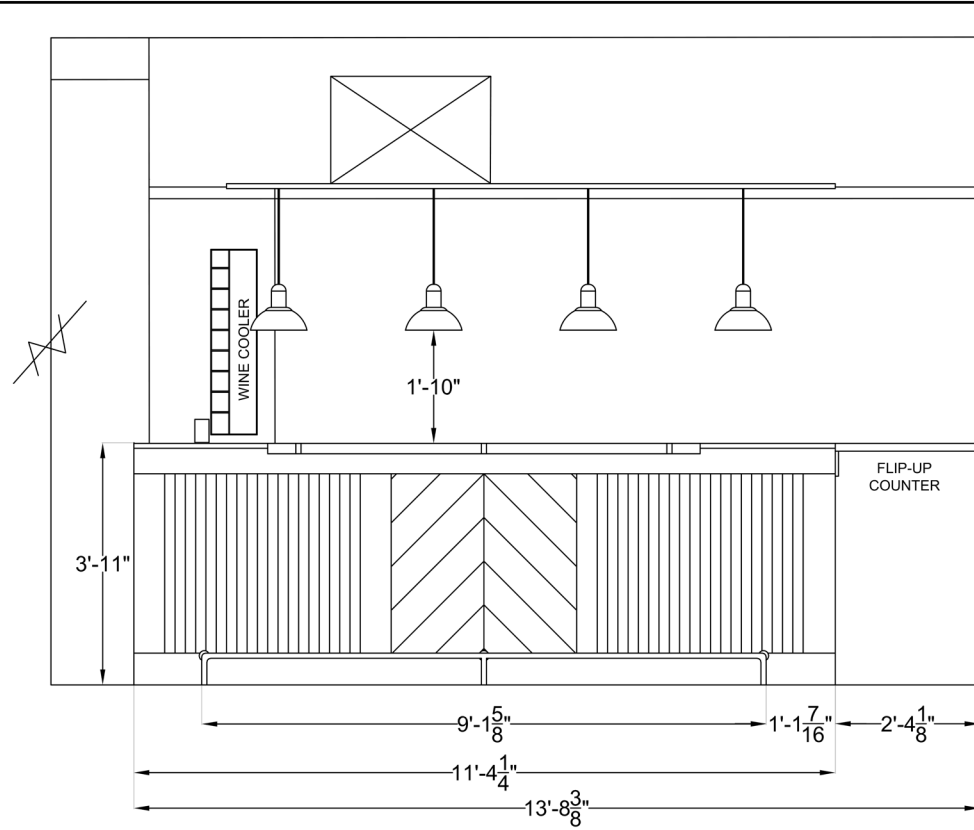
BAR FACADE FRONT ELEVATION
