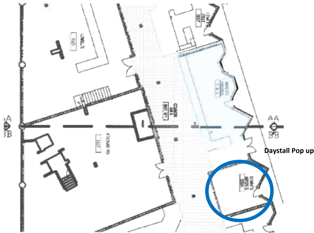
Site Plan—Arcade #4
