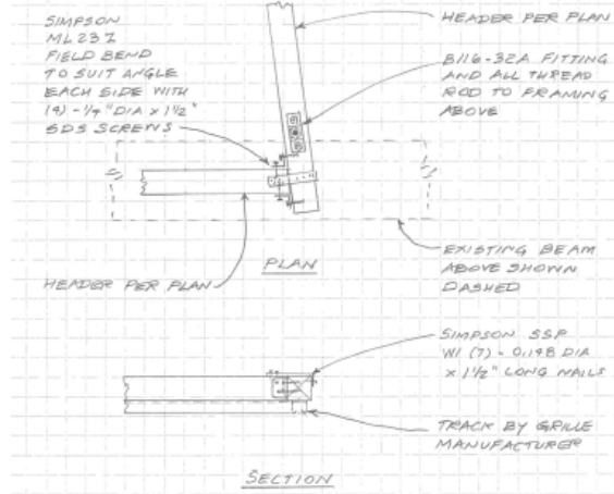
SK-2 PARTIAL ROOF FRAMING PLAN S2.0
