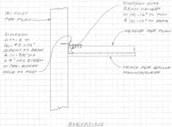
SK-1 TYP TRACK SUPPORT DETAIL S2.0
