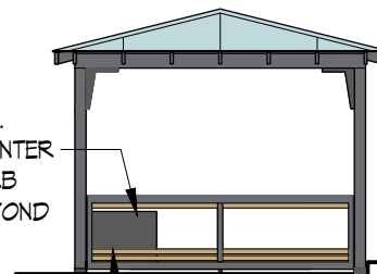
SECTION DETAIL
