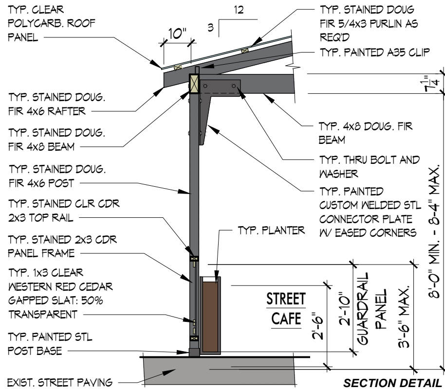
SECTION DETAIL
