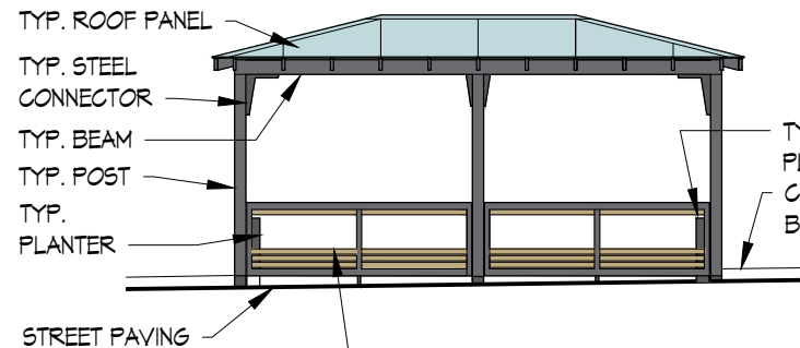
STREETSIDE ELEVATION
