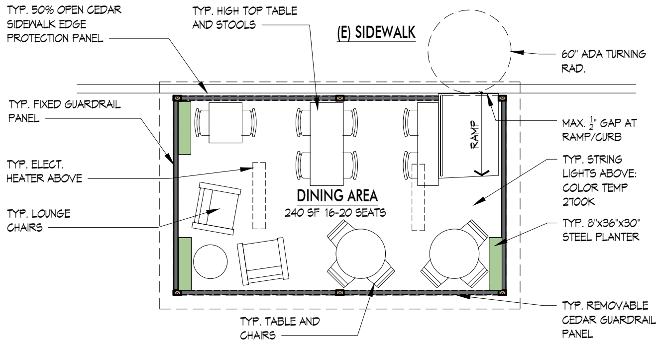
PROPOSED FURNISHING PLAN
