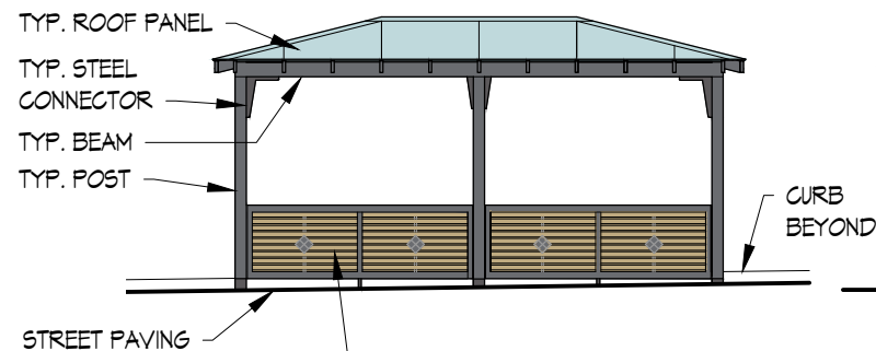
STREETSIDE ELEVATION
