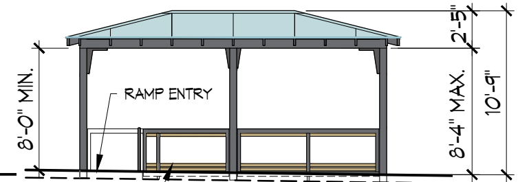
STREETSIDE VIEW OF EXISTING STREET CAFE / FISHER BUILDING
