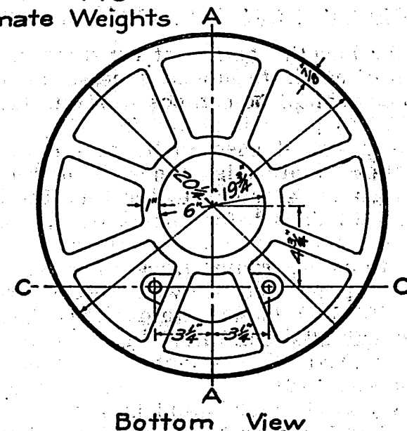
STANDARD VALVE CHAMBER COVER
