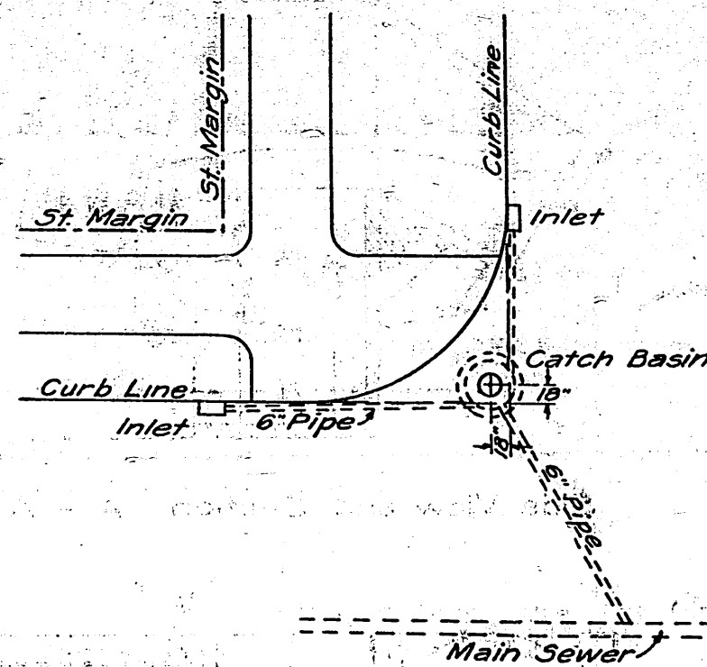
CATCH BASIN LOCATION
