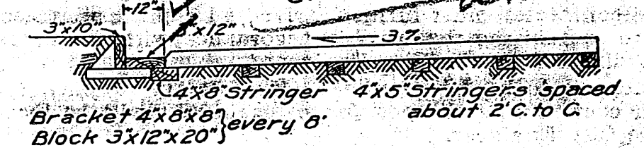
Section of Planking Type B
