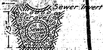
SEWER SUB DRAIN
