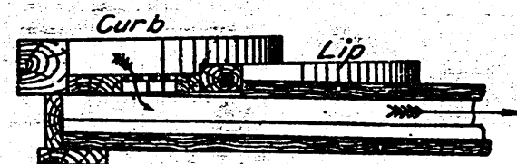
Section SPECIAL BOX DRAIN
