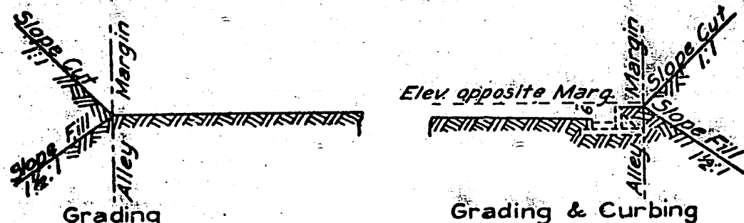
HALF SECTION OF ALLEY
