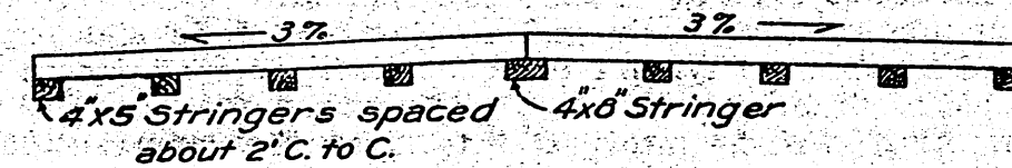
Section of Planking Type A
