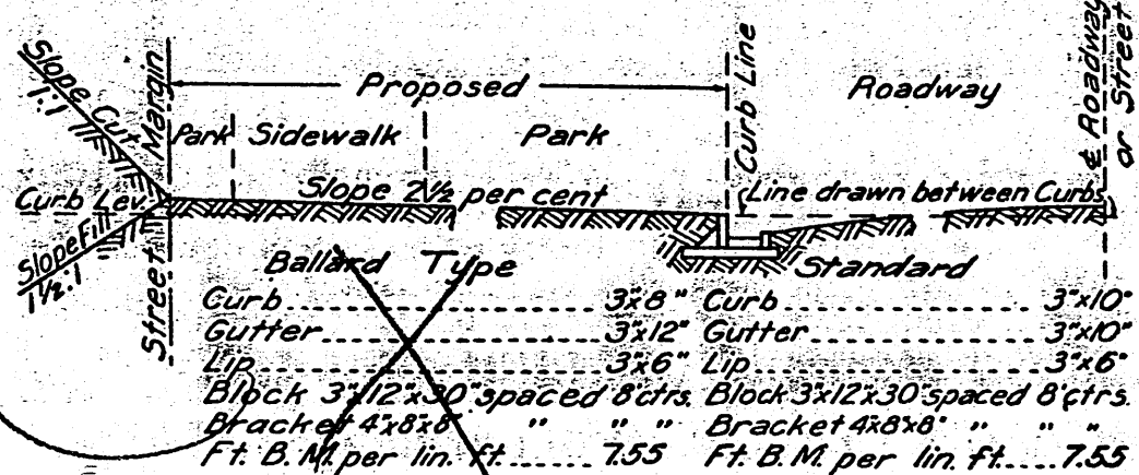
HALF SECTION GRADING & CURBING
