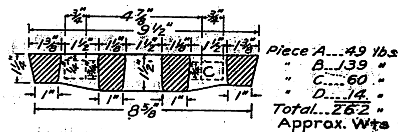
Section of Grate at Y-Y
