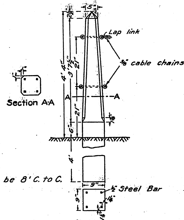
CHAIN FENCE WITH CONCRETE POST
