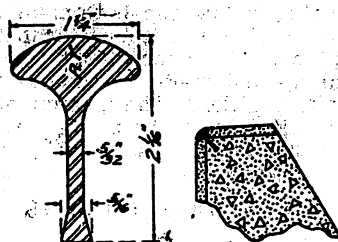
Detail Section Armor CURBING
