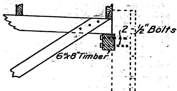
Cap Support on Wood Bulkhead
