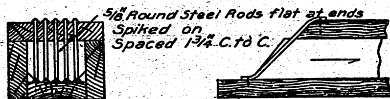
BOX DRAIN SCREEN
