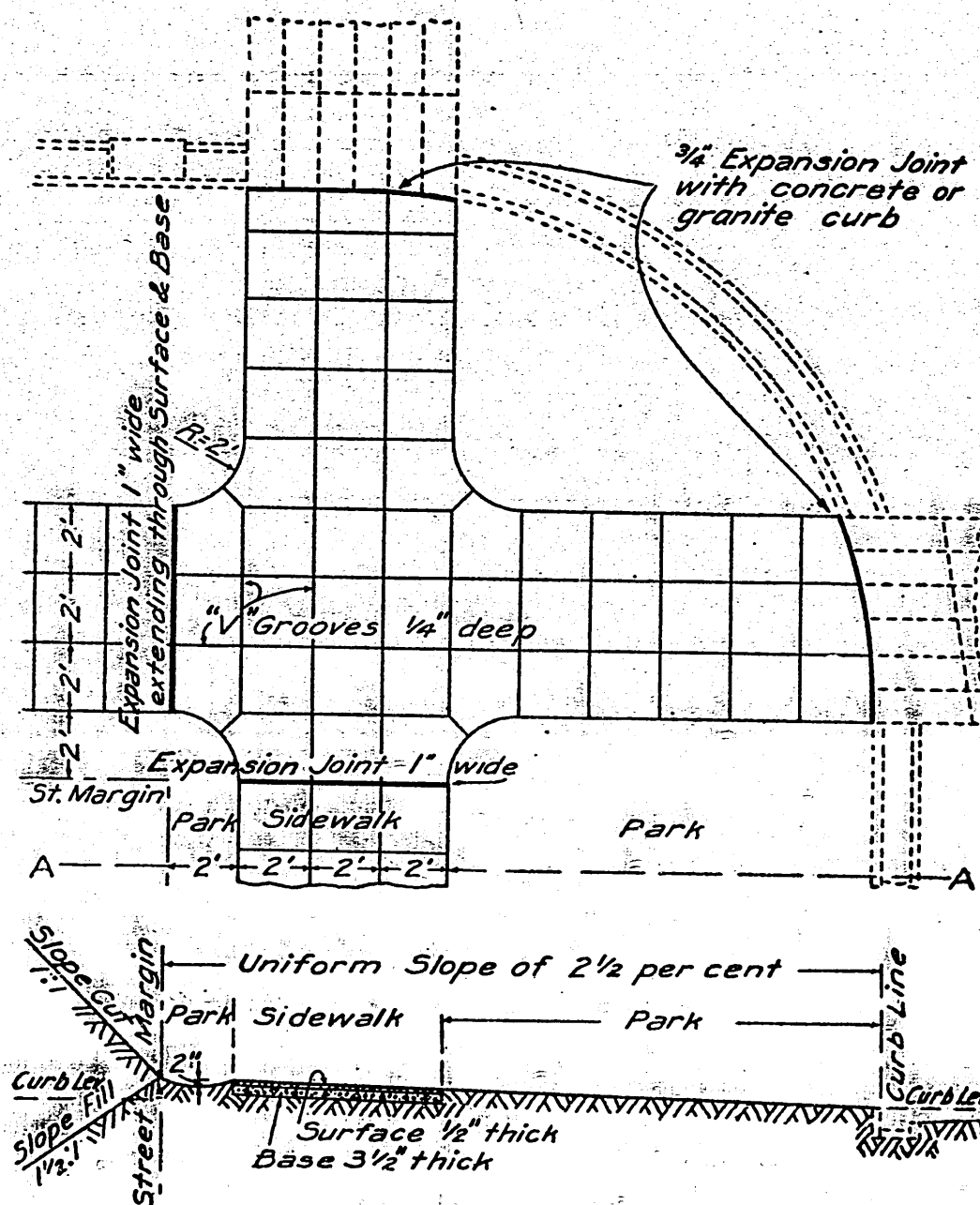
Section A-A Concrete Sidewalk Intersection
