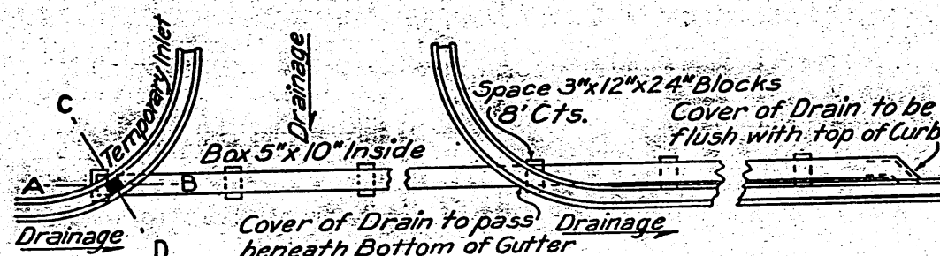
BOX DRAIN SCREEN
