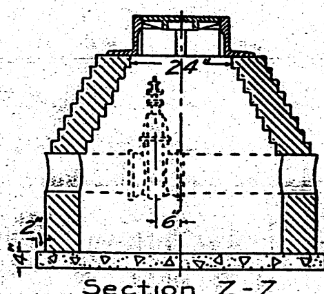
Section 7-7
