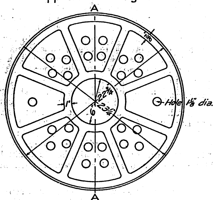
Bottom View
