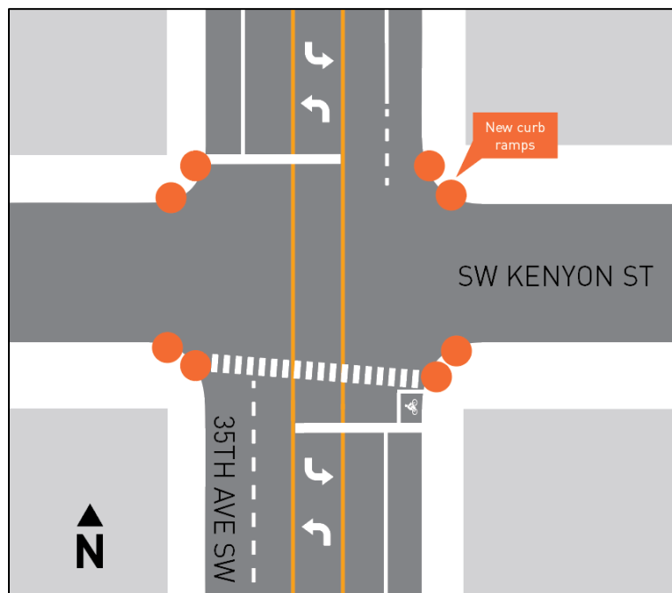
Improvements at 35th Ave SW/SW Kenyon St. Image not to scale.
