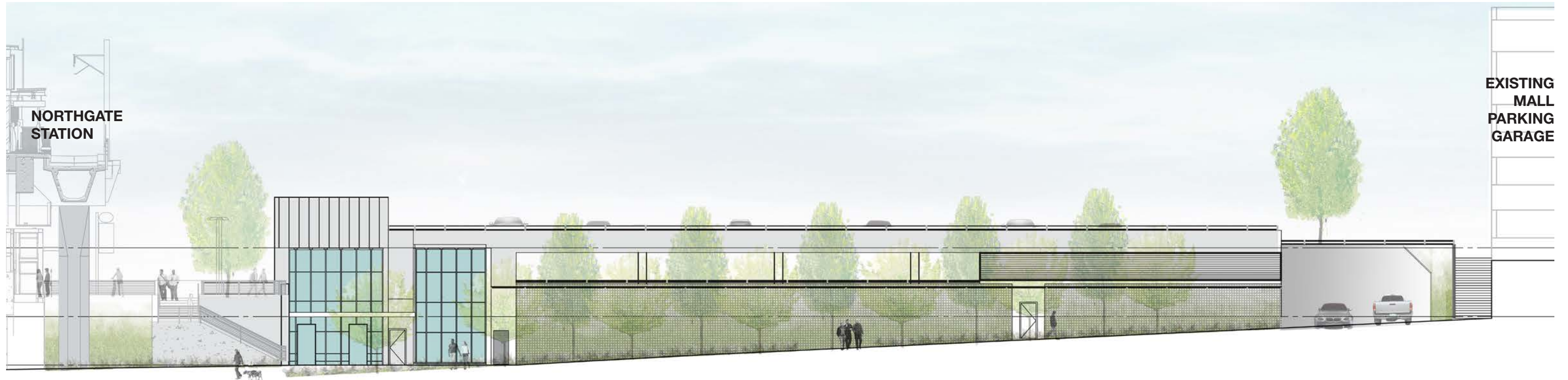
SOUTH ELEVATION - Looking from NE 103RD ST
