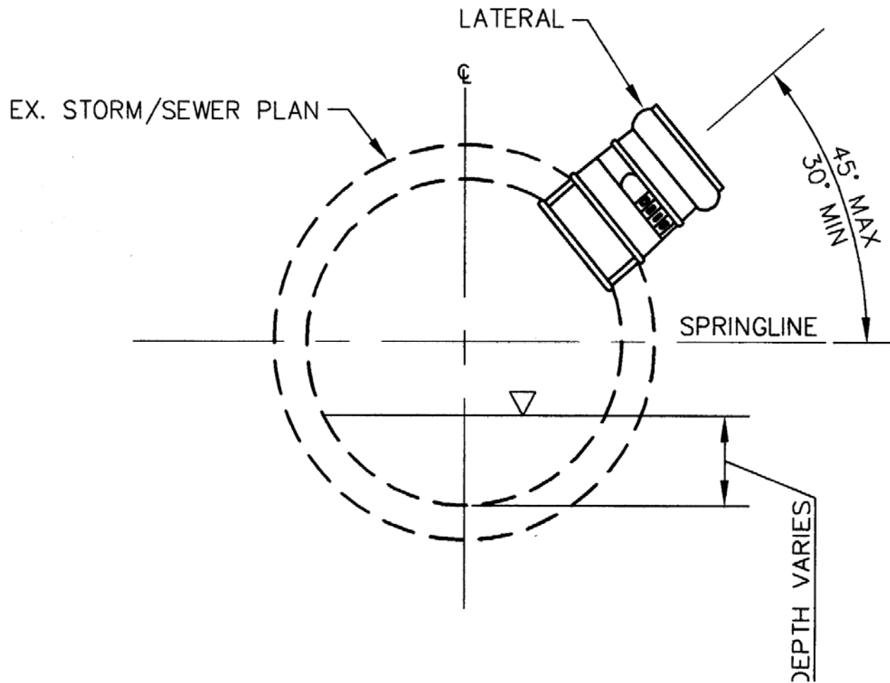
Figure 1 Cross Section
