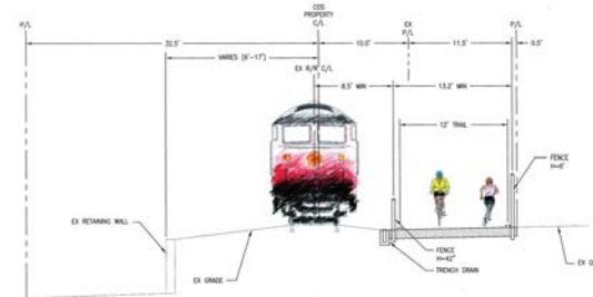
Section H NW 54th St - 26th Ave. to 28th Ave. Not to Scale
