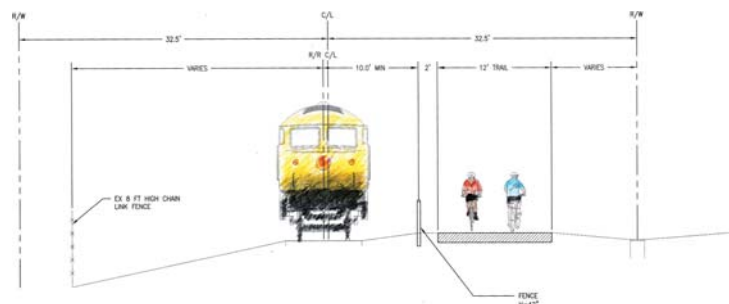
Section I NW 54th St - 28th Ave. to 30th Ave. Not to Scale
