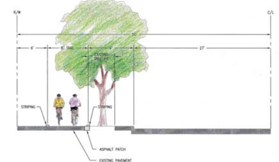
Section G NW Market St. 26th Ave. NW to 28th Ave. NW Not to Scale
