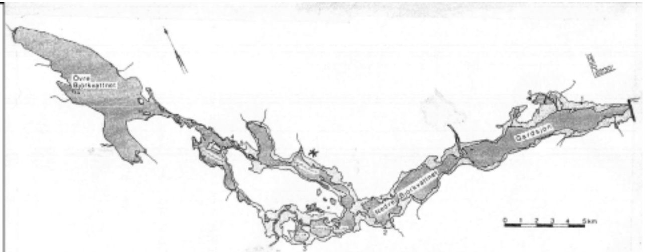
Figure 4. Map (upper) of Gardiken Reservoir system (fine stippling) in northern Sweden (19°50'N, 65°30'W) formed by impoundment of a chain of lakes (dark hatching). * shows approximate photograph (A, B, C) site. A: spring at lowest level, shore ice-covered. B: early summer, still at lowest level, shore exposed. C: late summer, high water level. Adapted from Nilsson (1981).
