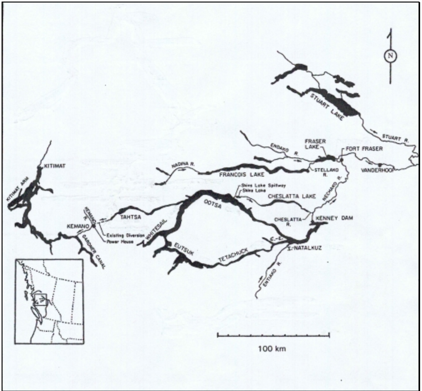
Figure 15. The Nechako Reservoir formed by Kenney Dam on the upper Nechako River, its six major depressions (Intata-Natalkuz, Ootsa, Tahtsa, Whitesail, Eutsuk and Tetachuck) and one minor depression (Chelasia-Euchu) named after the former lakes and connecting rivers. Adapted from Hartman (1996).
