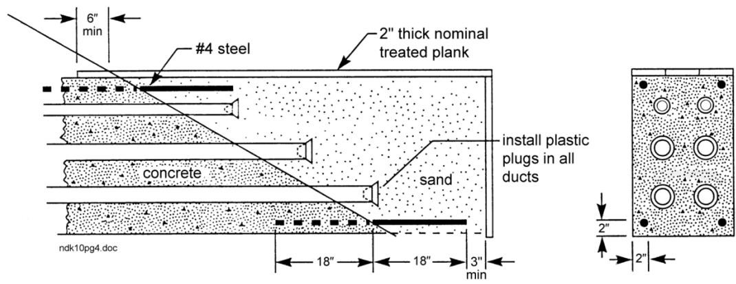
Figure 5.2.2. Temporary Termination
