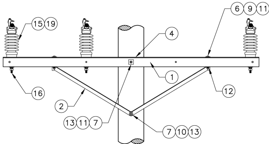
Figure 3.3d.397.5 kcmil and 954 kcmil ACSR Lower Gain
