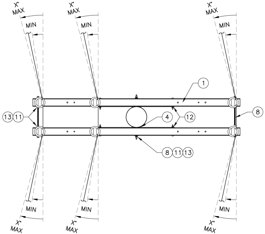
Figure 3.3c. #4 AWG Copper Lower Gain
