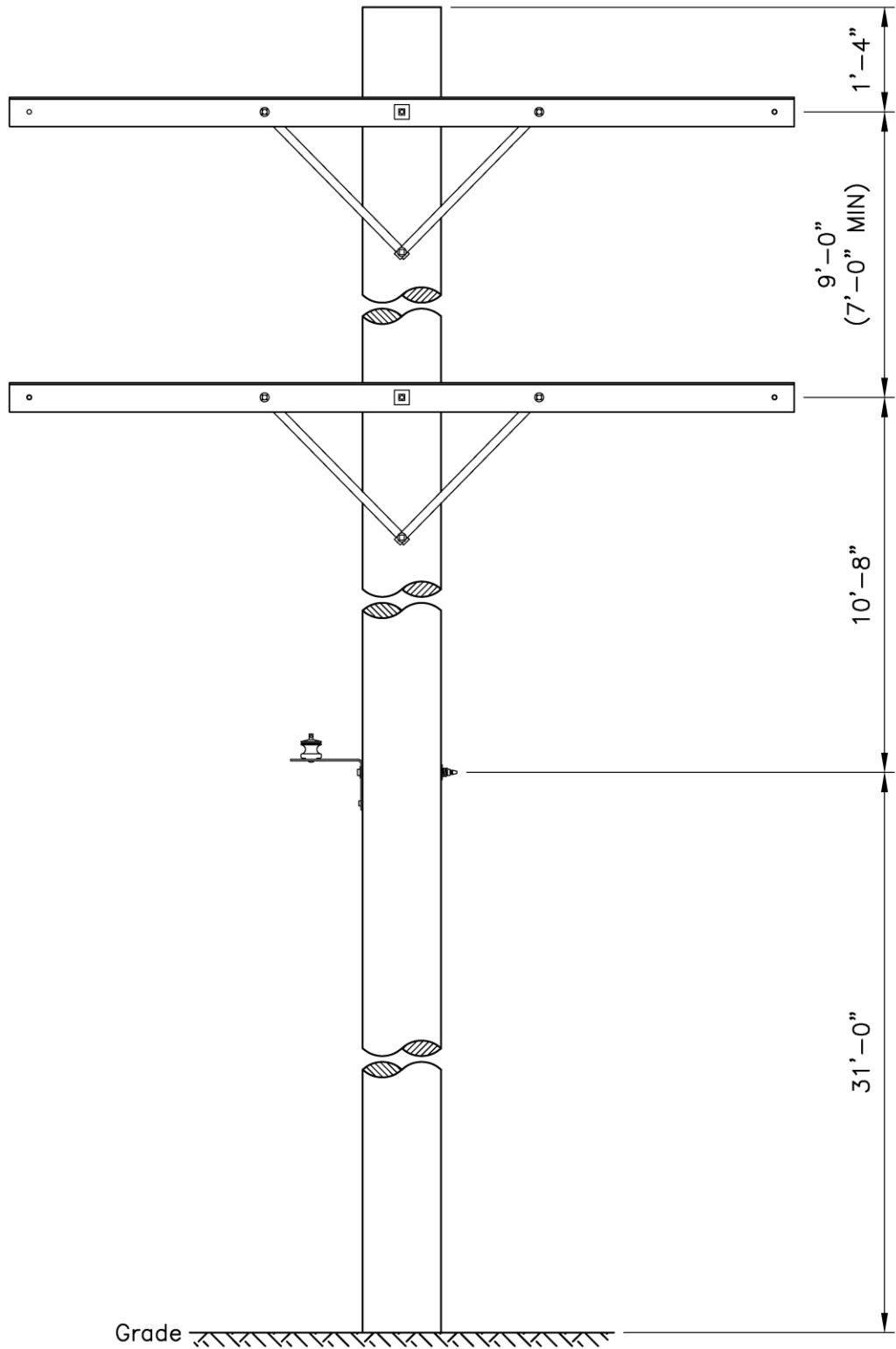
Figure 3.1a. Parallel Angle Configuration
