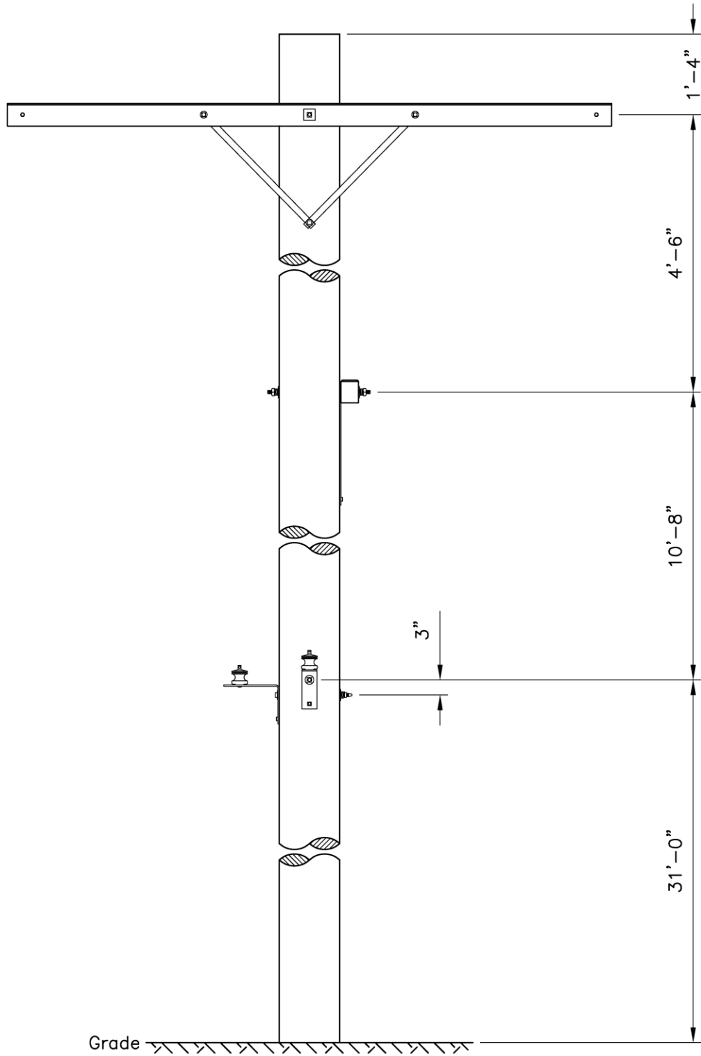
Figure 3.1b. Perpendicular Angle Configuration
