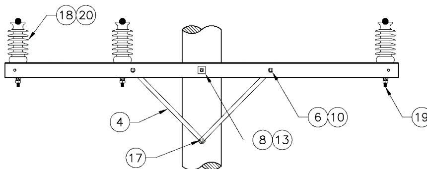
Figure 3d. #4 AWG Copper Lower Gain of a Three-Phase Multi-Gain Tangent Pole Top Assembly
