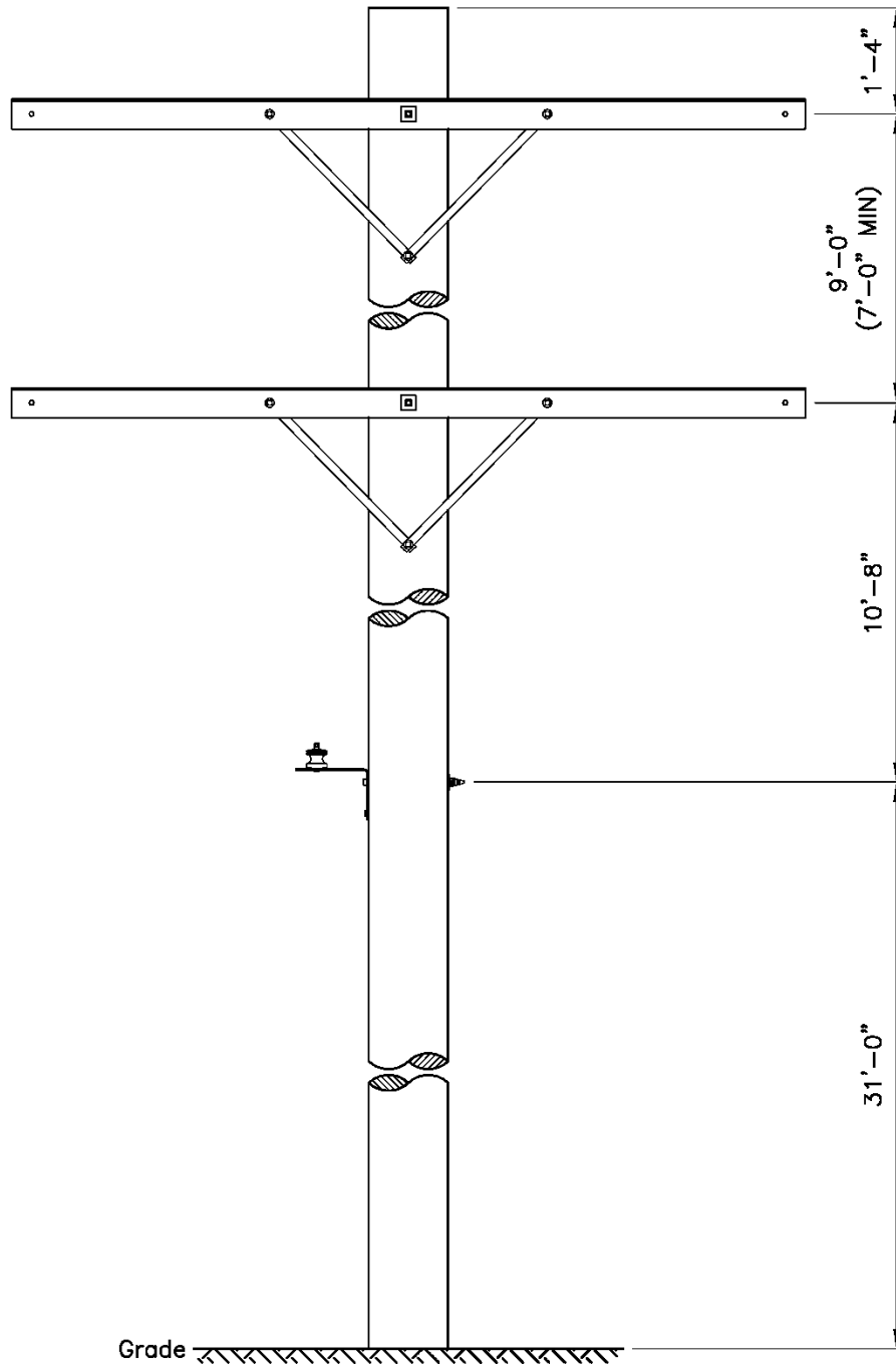
Figure 3a. Parallel Tangent Configuration
