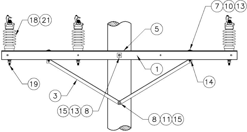
Figure 3h. Grade B 954 kcmil ACSR Lower Gain of a Three-Phase Multi-Gain Tangent Pole Top Assembly
