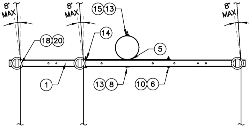
Figure 3c. Allowable Line Angle Range for #4 AWG Copper Tangent Lower Gain
