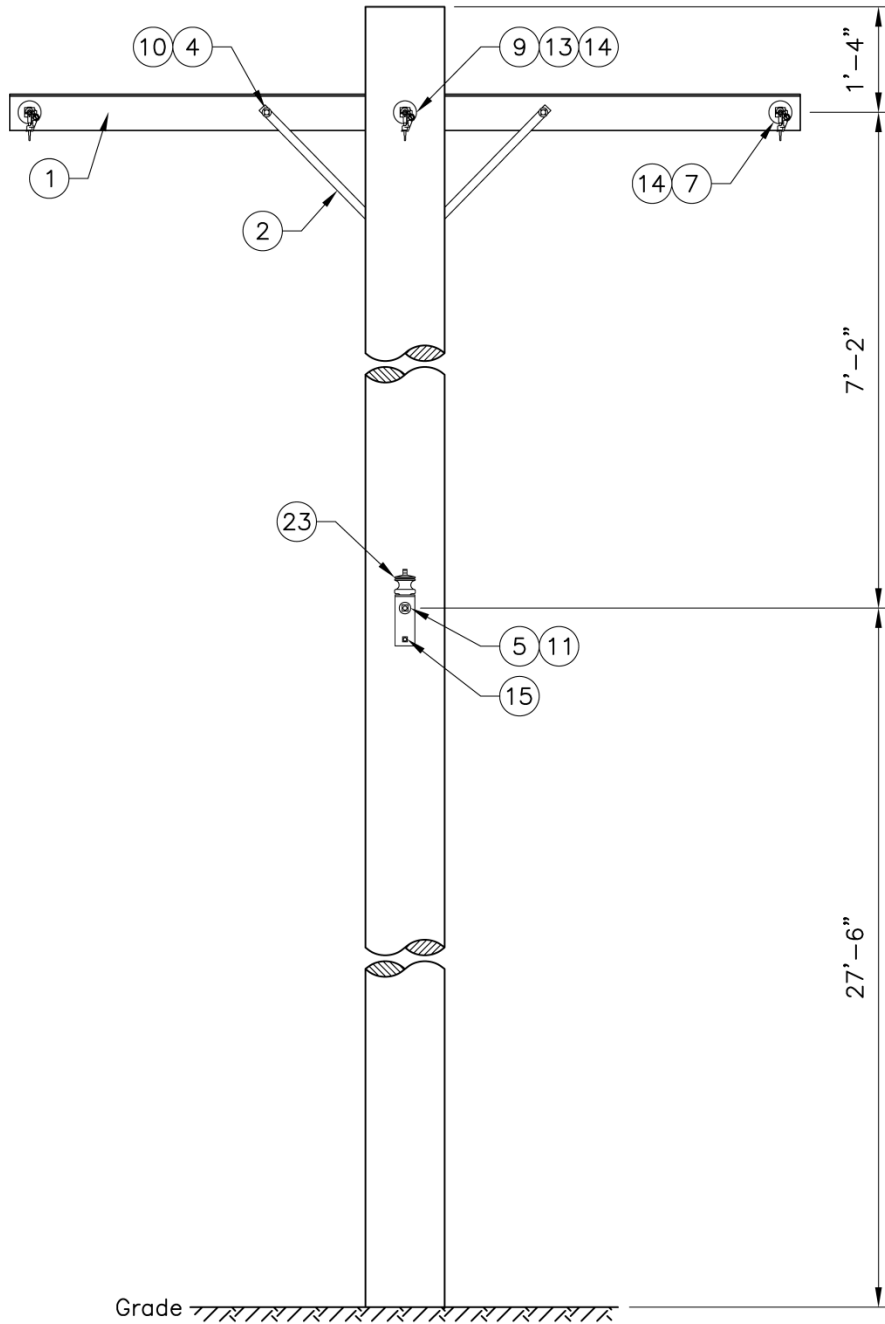
Figure 3b. Three-Phase Single Deadend Pole Top Assembly for View Areas, Side View
