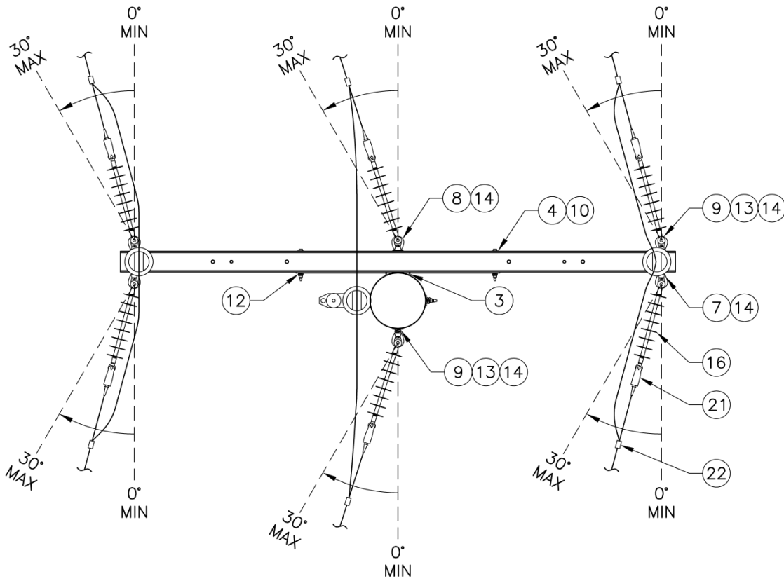
Figure 3c. Allowable Line Angle Range for Double Deadend View Pole
