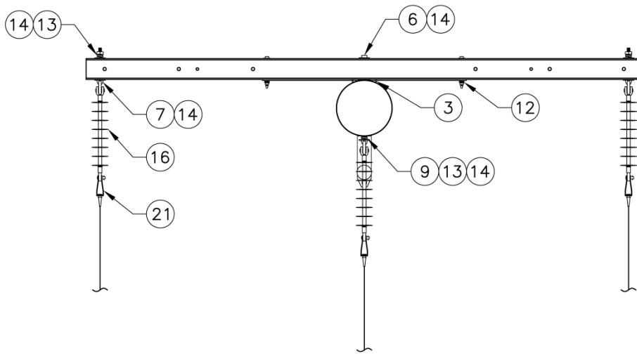
Figure 3a. Three-Phase Single Deadend Pole Top Assembly for View Areas, Top View
