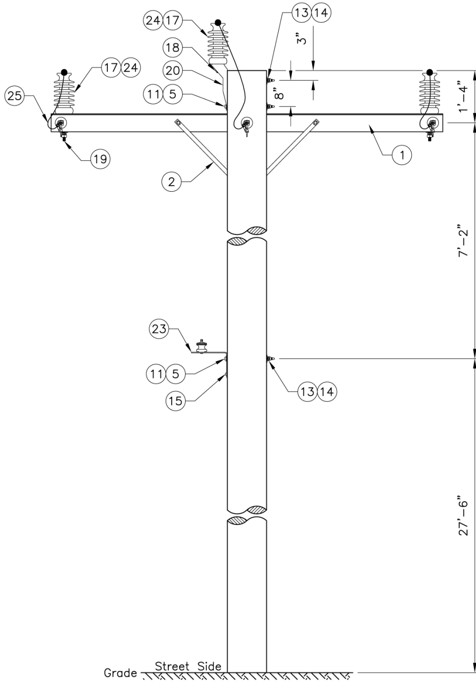
Figure 3d. Three-Phase Double Deadend Pole Top Assembly for View Areas
