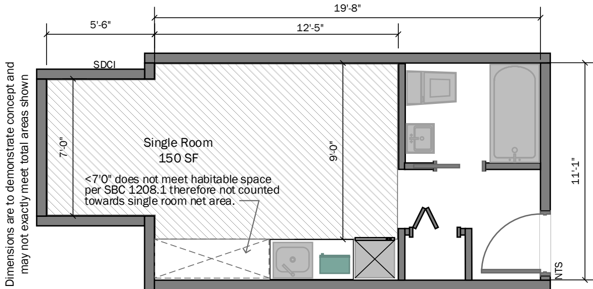
FIGURE 5: EXAMPLE OF SINGLE ROOM USING MINIMUM HABITABLE AREA
