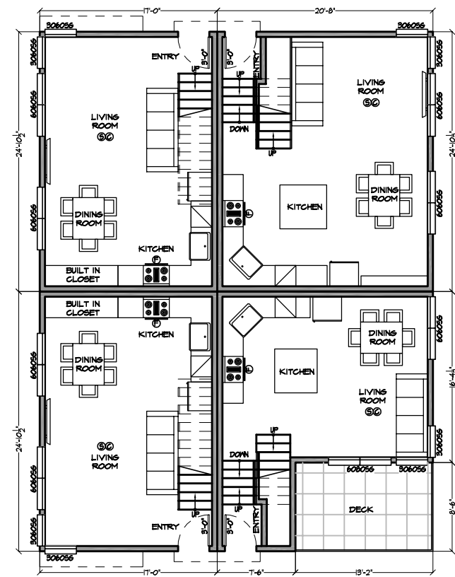
FIRST FLOOR PLAN BUILDING 2 - UNITS E-H
