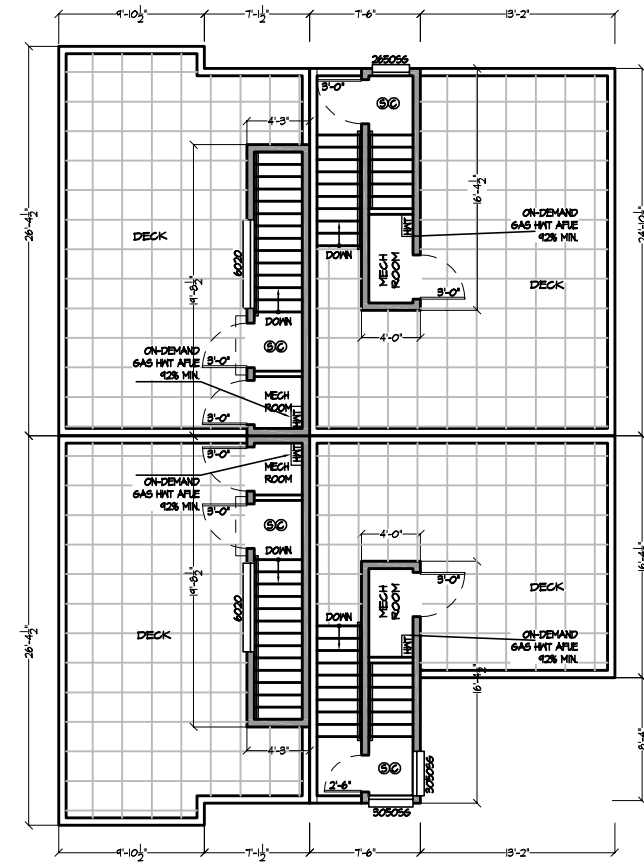
ROOF DECK PLAN BUILDING 2 - UNITS E-H
