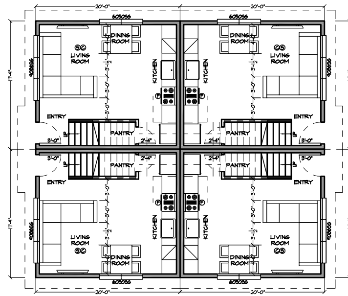
FIRST FLOOR PLAN BUILDING 1 - UNITS A-D
