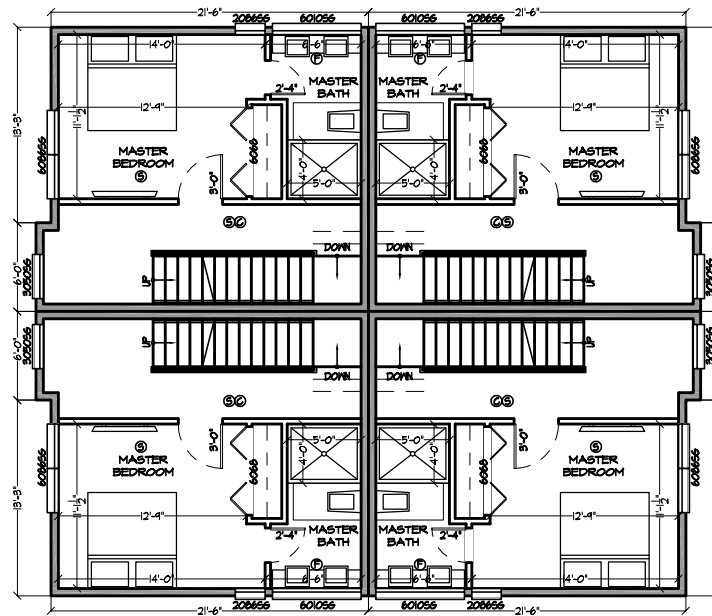
THIRD FLOOR PLAN BUILDING 1 - UNITS A-D
