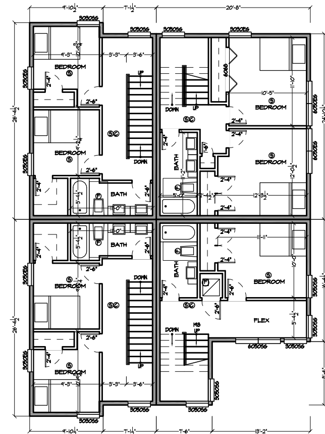
SECOND FLOOR PLAN BUILDING 2 - UNITS E-H
