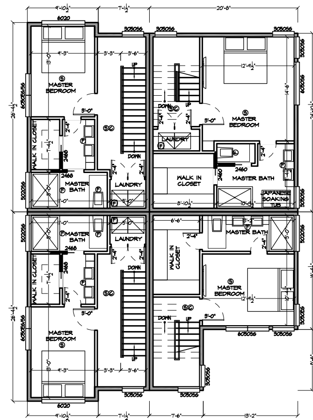
THIRD FLOOR PLAN BUILDING 2 - UNITS E-H
