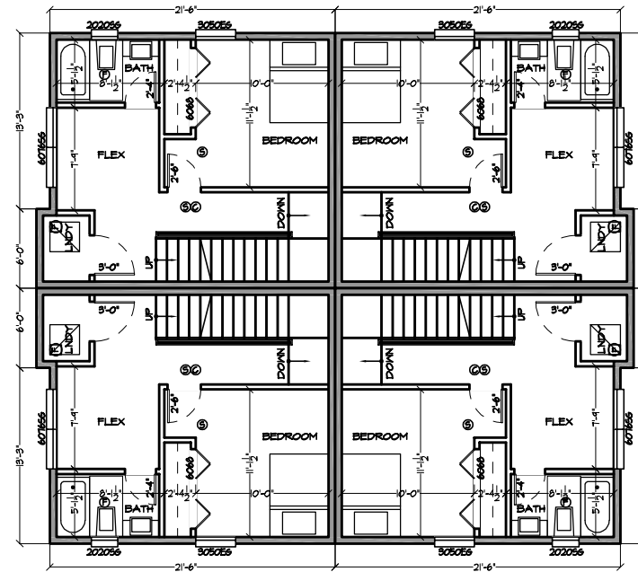
SECOND FLOOR PLAN BUILDING 1 - UNITS A-D
