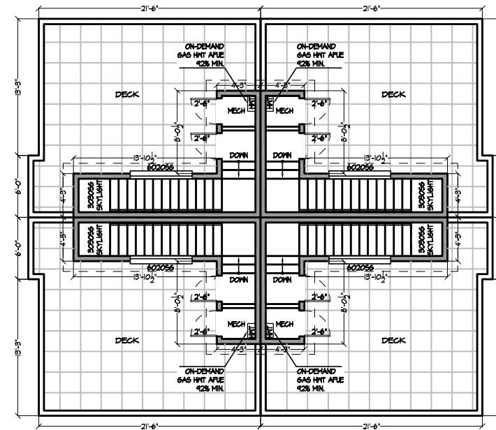
ROOF DECK PLAN BUILDING 1 - UNITS A-D
