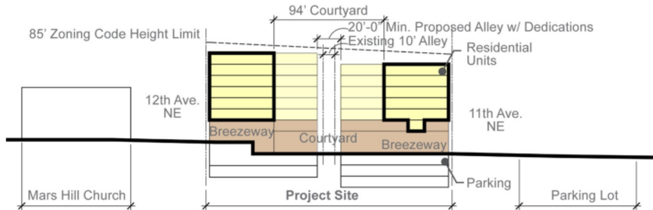
Section Alternative 5 (Preferred)
