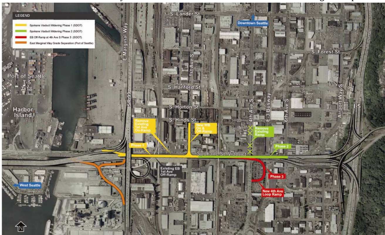
South Spokane Street Viaduct Widening Project Plan
